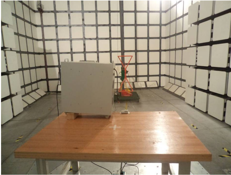
Below 1 GHz: Radiated Emissions View
