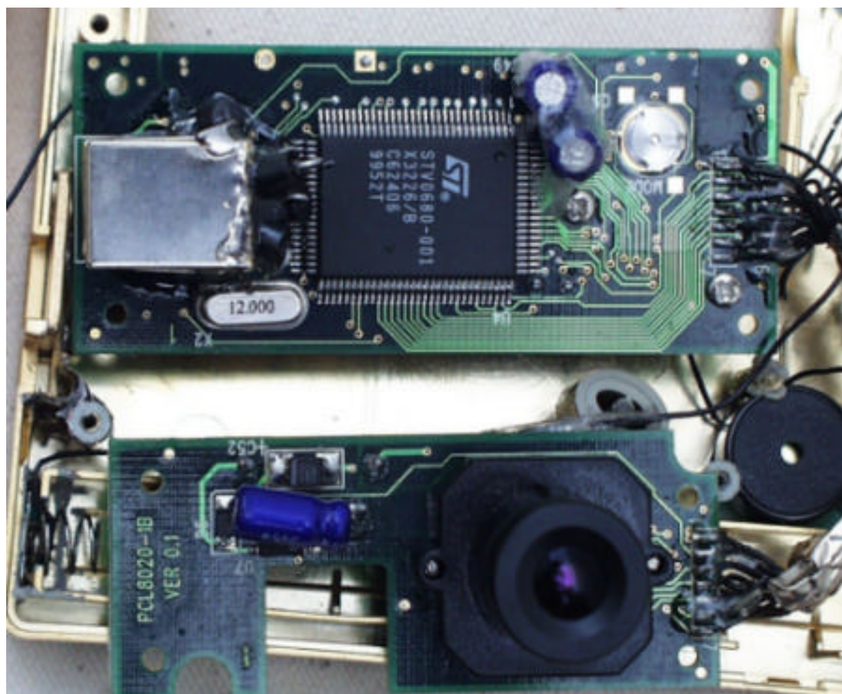
FCC ID: OYZPCL8020 FRONT VIEW OF THE PRINTED WIRING BOARD
