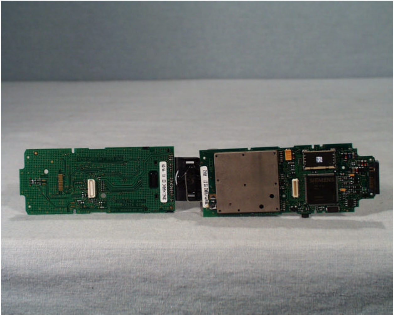
Back view of the radio board and keypad board
