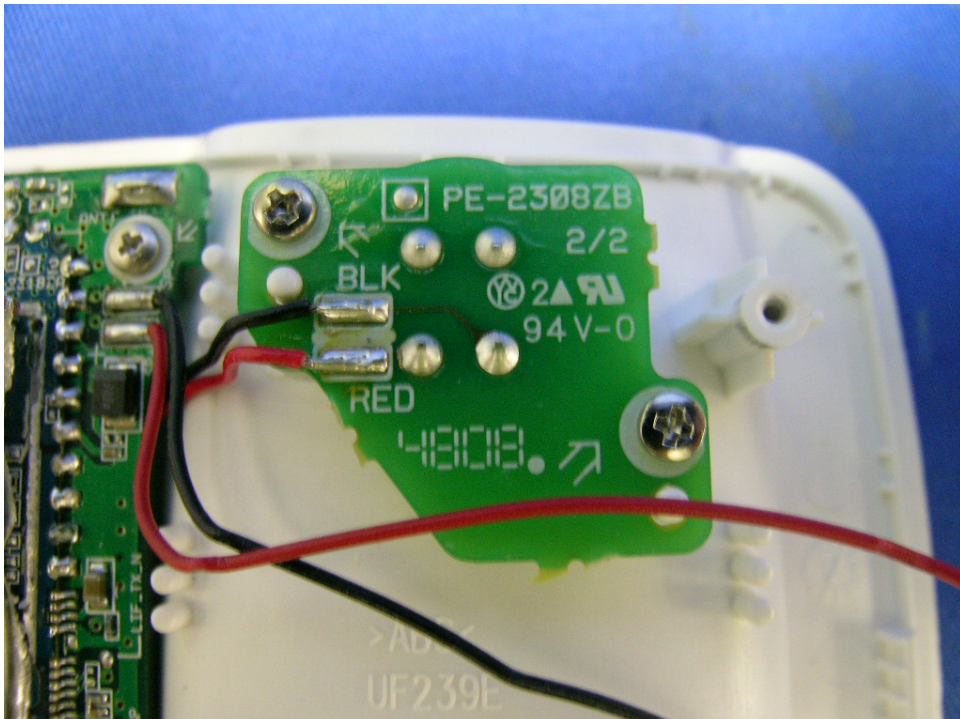
Base Unit PCB of Handset Location Button rear side
