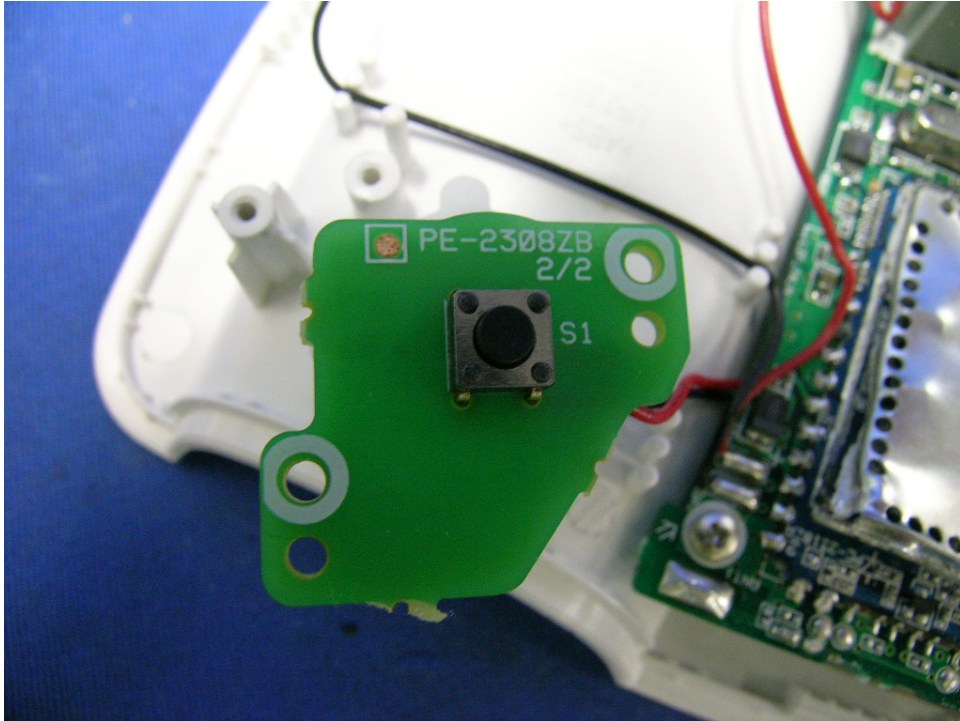
Base Unit PCB of Handset Location Button front side
