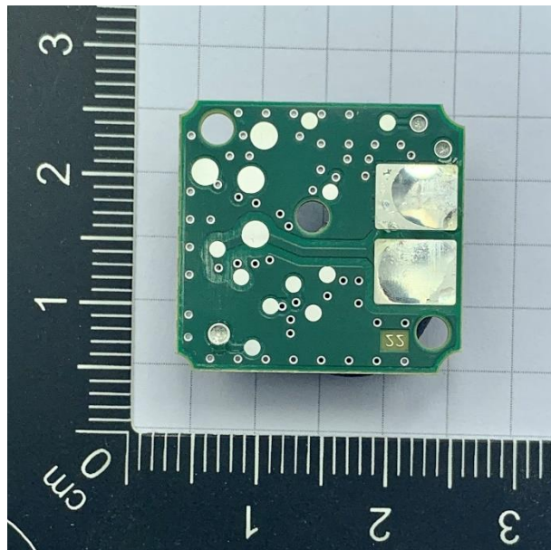
PCB bottom view
