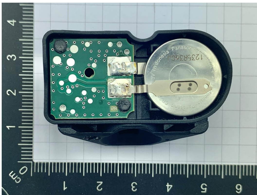
assembly with battery and housing
