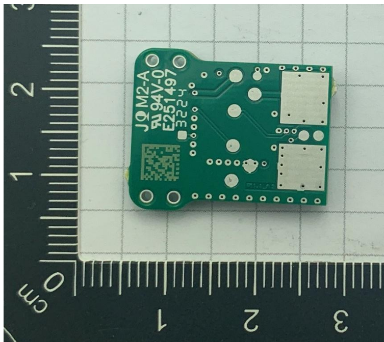
PCBA bottom view
