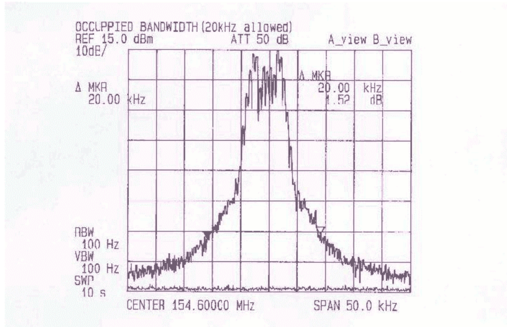
PLOT 1 OCCUPIED BANDWIDTH FOR 150 MHz, 15 dBm PEAK CARRIER LEVEL
