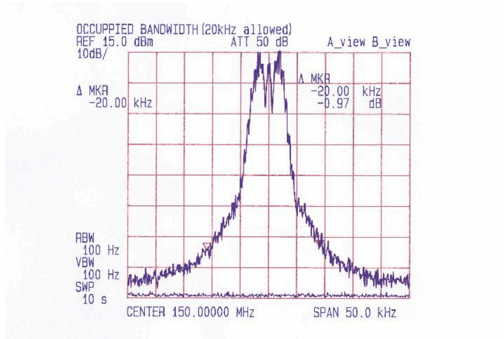
PLOT 1 OCCUPIED BANDWIDTH FOR 150 MHz, 15 dBm PEAK CARRIER LEVEL
