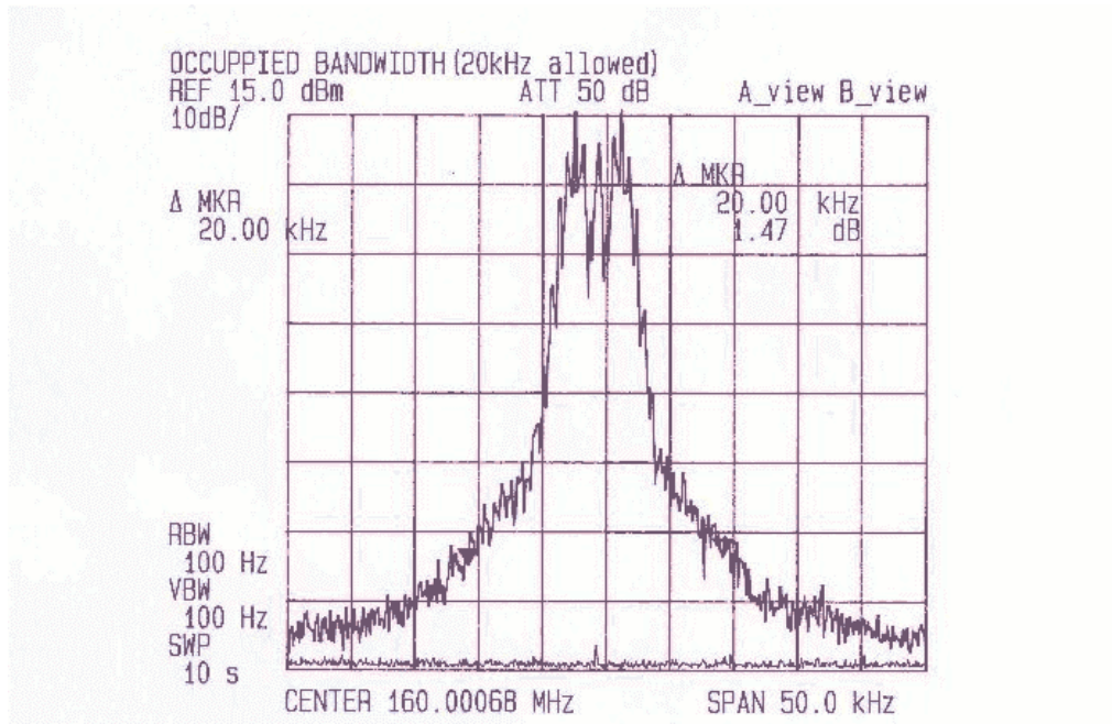
PLOT 3 OCCUPIED BANDWIDTH FOR 160 MHz, 15 dBm PEAK CARRIER LEVEL
