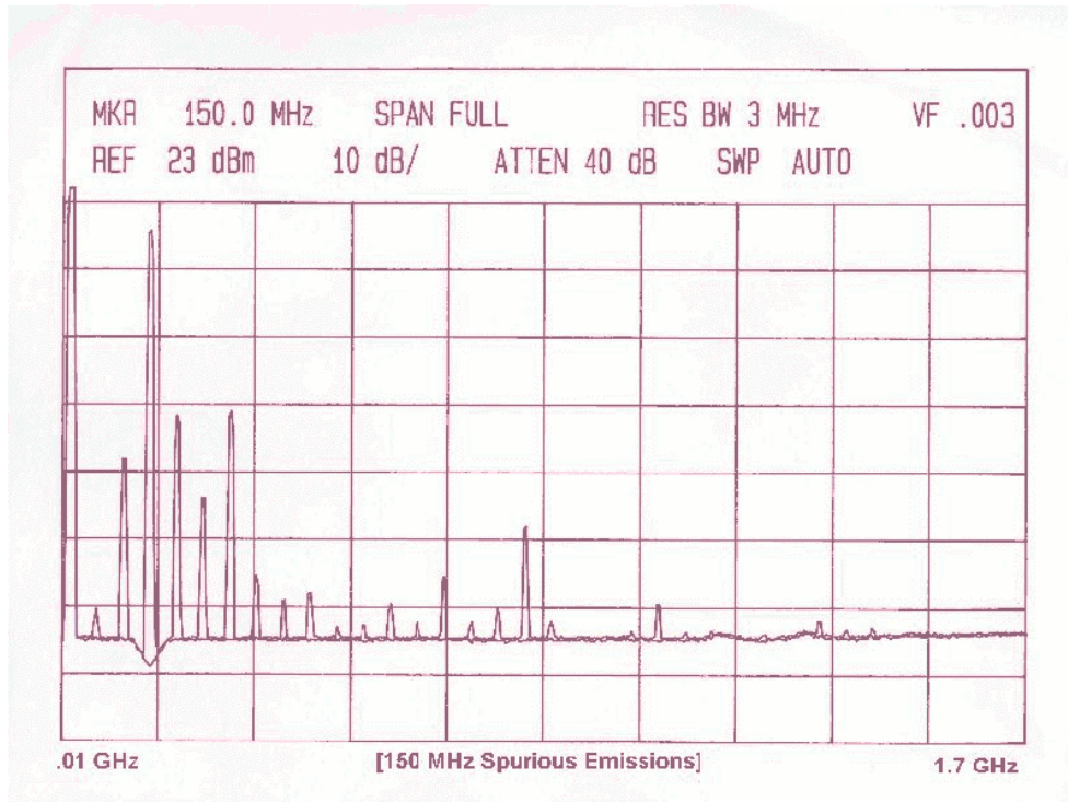
PLOT 5 SPURIOUS EMISSIONS FROM 150MHz
