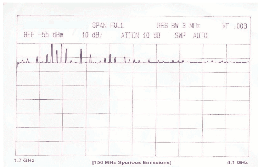
PLOT 6 SPURIOUS EMISSIONS FROM 150MHz
