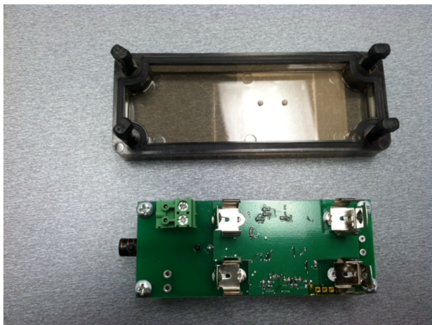
Figure 4: MWT12 PCB battery side
