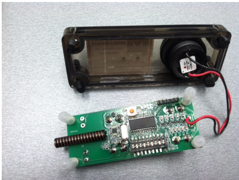
Figure 1: MWT A12 PCB component side
