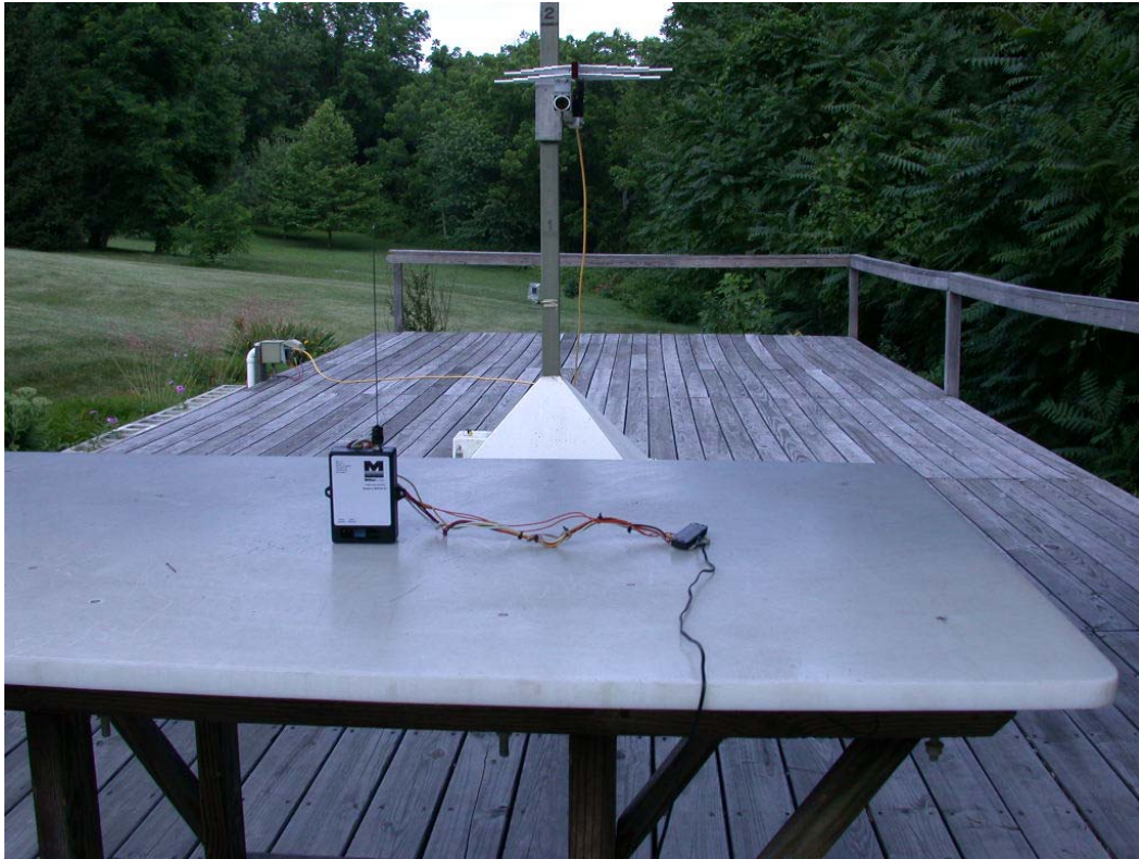
Radiated Test Set-up for Receiver
