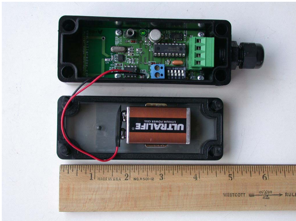
Transmitter, Open View
