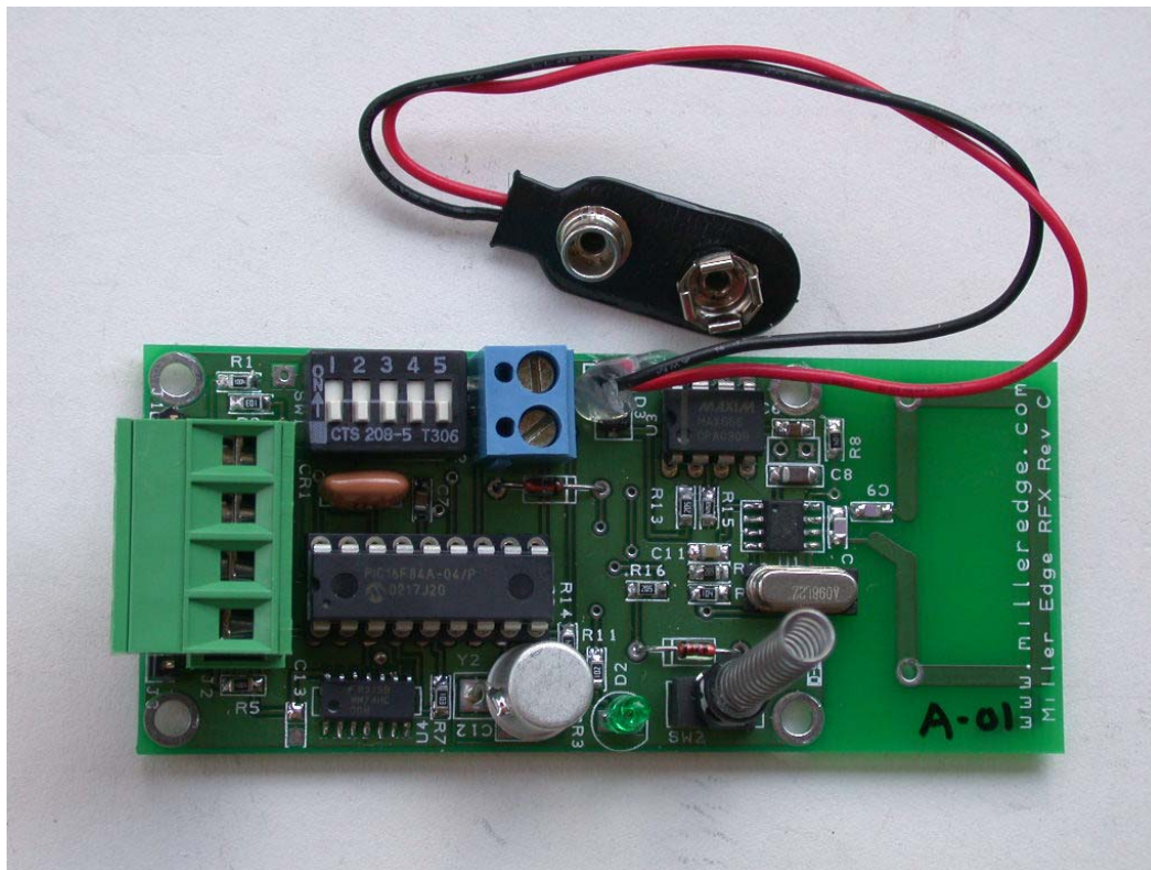
Transmitter, Component Side of Printed Circuits Board
