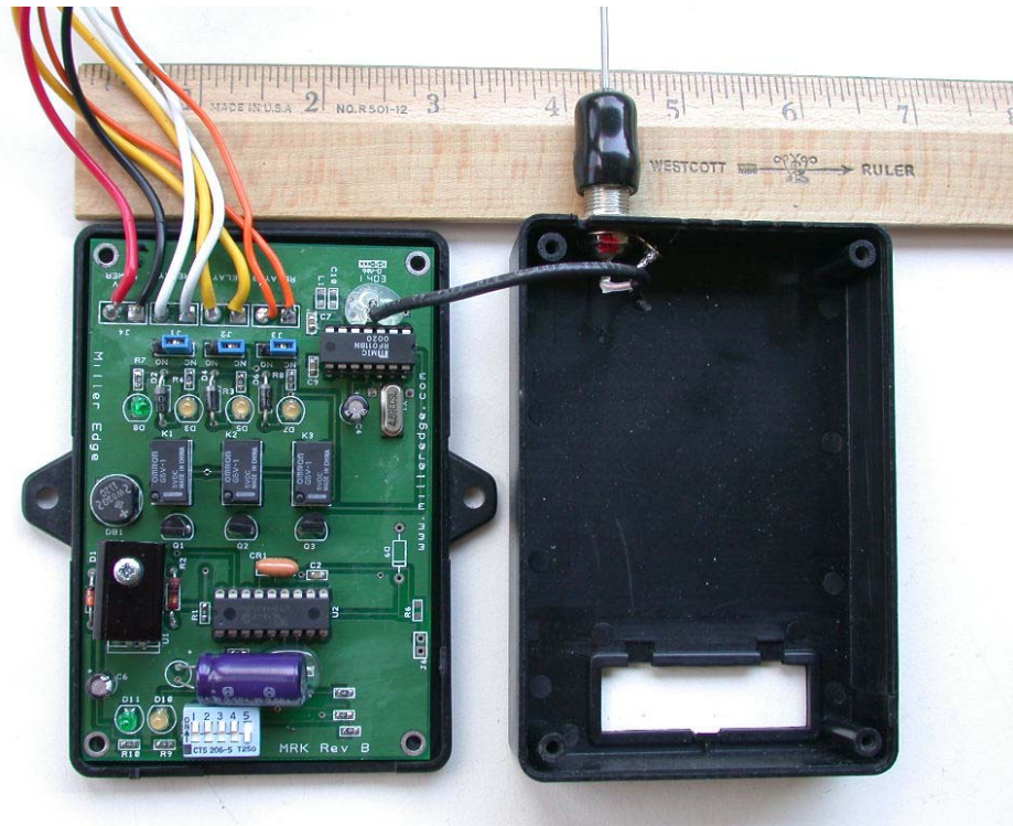
Receiver, Open View
