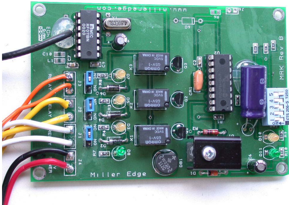
Receiver, Circuit Side of Printed Circuits Board
