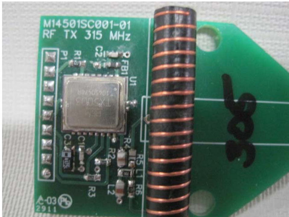
RF Component Side
