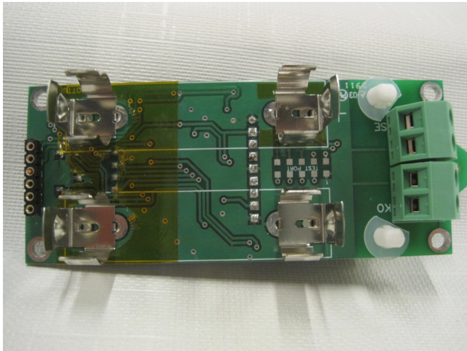
Main with Batteries Removed
