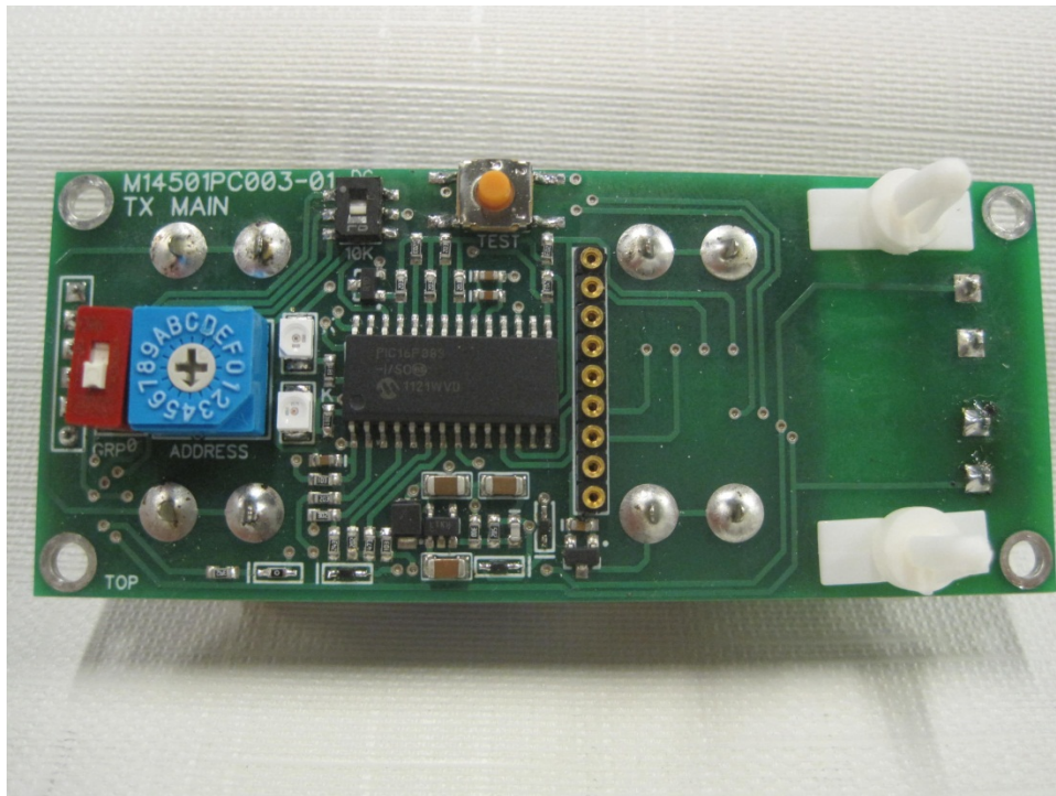
Main with RF Board Removed
