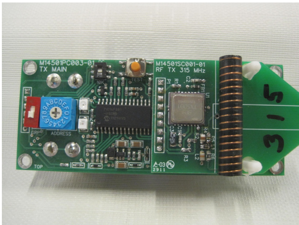
Main and Transmitter
