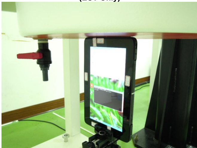
Secondary Portrait with 0 cm Gap (EUT Only)
