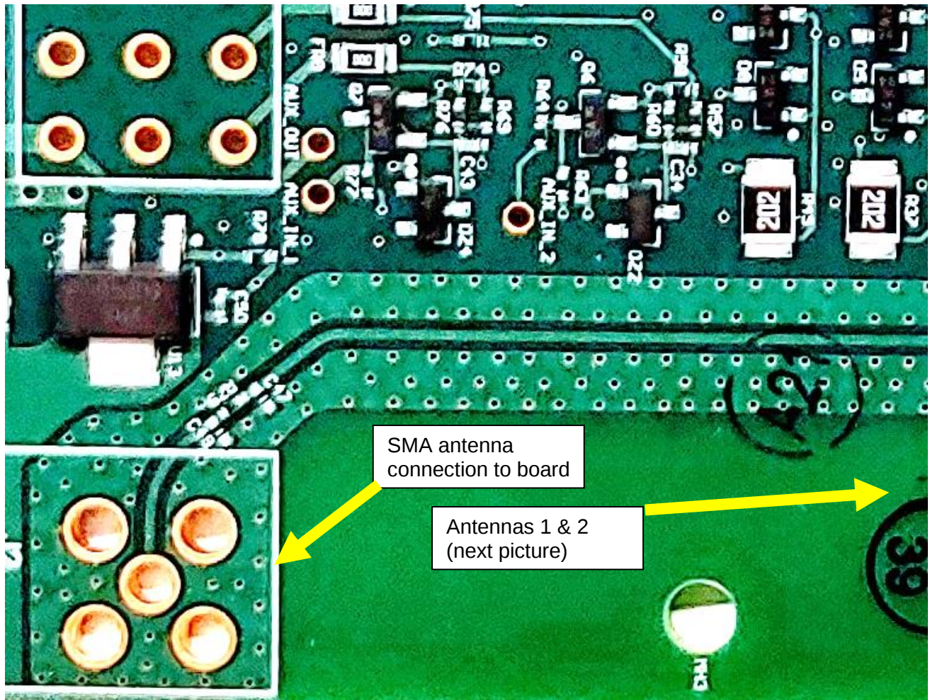
PRECOLink closeup part 1. SMA connector traces, antenna 3
