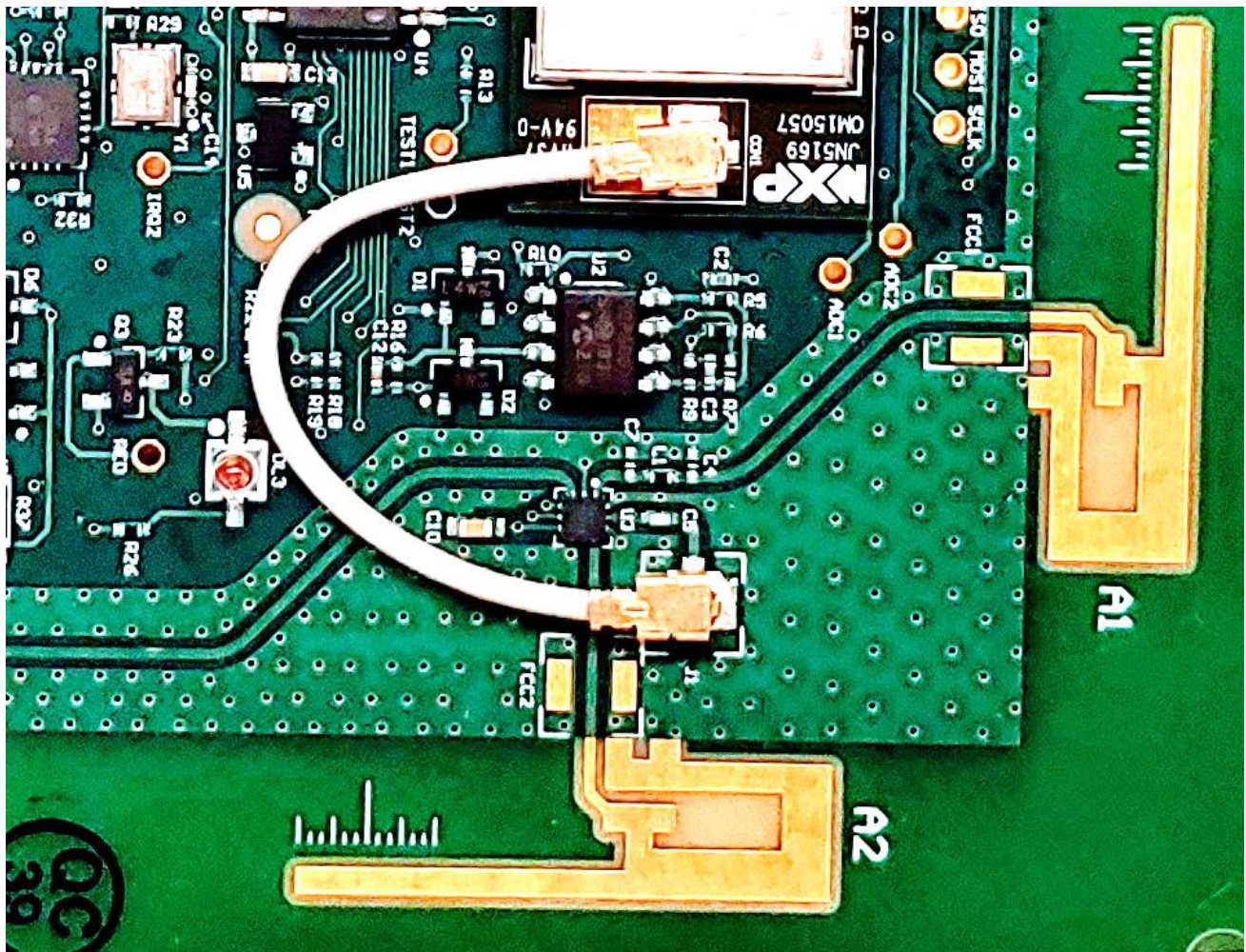
PRECOLink closeup part 2. Antenna 1 & 2
