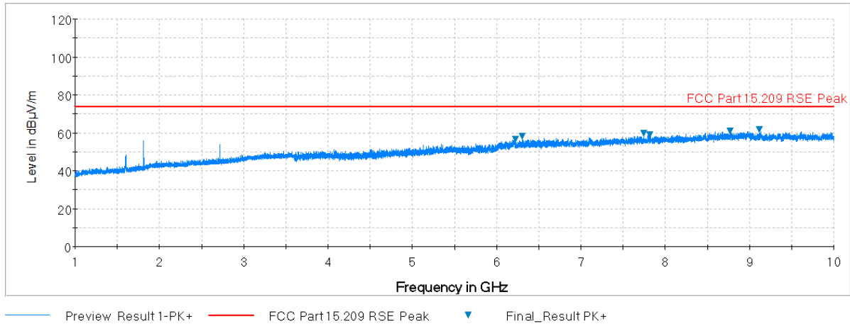
Plot 7-18. Radiated Spurious Plot above 1GHz (Low Channel, Ant. Pol. H)
