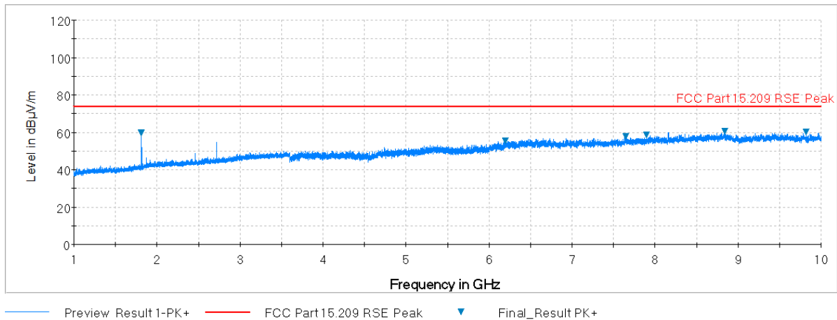
Plot 7-19. Radiated Spurious Plot above 1GHz (Low Channel, Ant. Pol. V)
