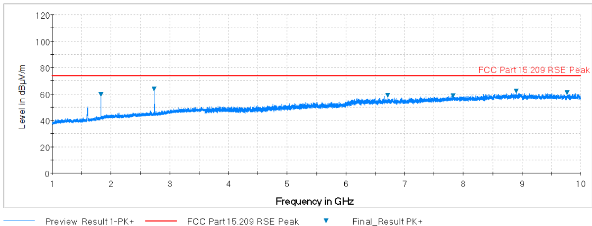
Plot 7-20. Radiated Spurious Plot above 1GHz (Mid Channel, Ant. Pol. H)
