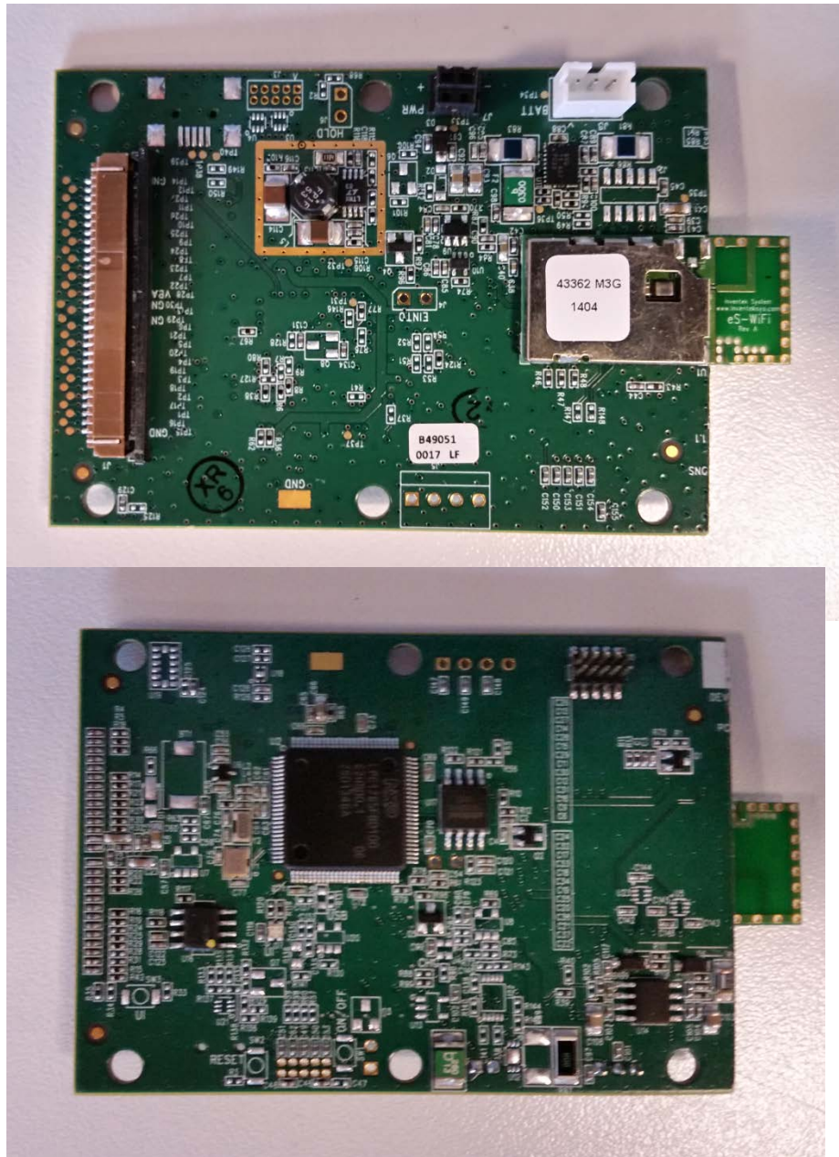
OXW-DS0028 WiFi Board (PA0021)
