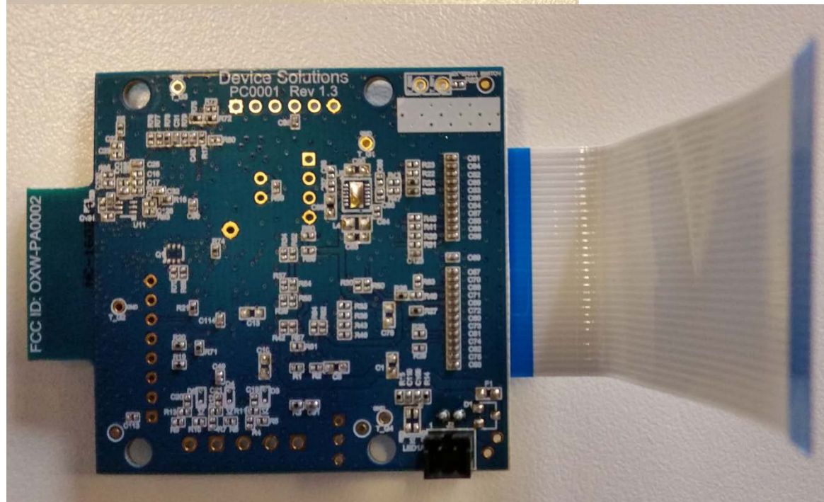
OXW-DS0028 900MHz Radio Board (PA0002)
