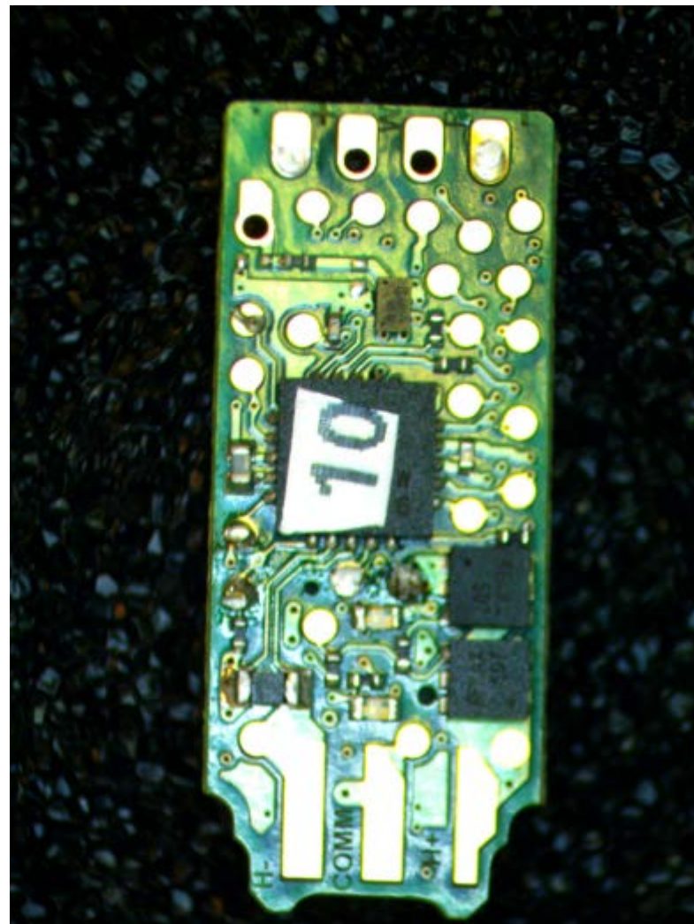
PCB photo bottom side A1006017RBT Rev 4.01
