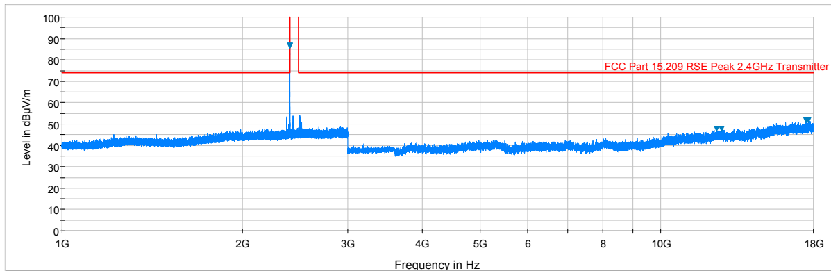
Plot 6-4. Radiated Spurious Plot above 1GHz (BTLE – Ch. 0, Ant. Pol. H)
