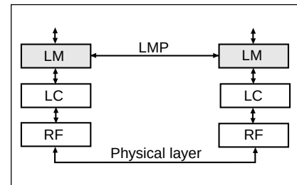
Figure 13. Link manager
