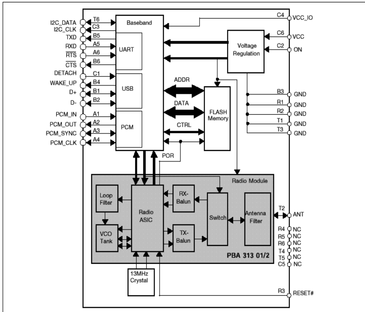
Figure 1. Block Diagram
