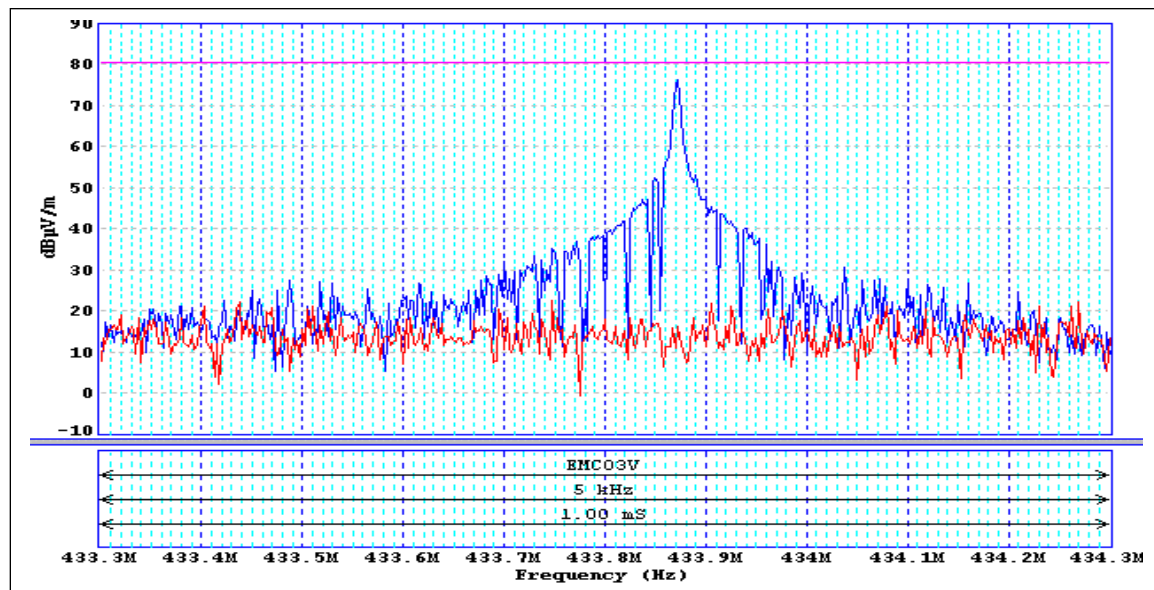
Fig.1. Fundamental emission spectrum of the EUT. Blue is with the EUT functioning and Red is the ambient. The field was measured with an EMCO 3143 broadband vertically polarized antenna located 3-m from the EUT. Note that this data is taken with peak detection. The quasi-peak field is required to be lower than the limit line shown (section 15.231)
