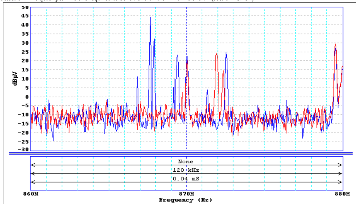
Fig.2. Second harmonic emission spectrum of the EUT. Blue is with the EUT functioning and Red is the ambient. The field was measured with an EMCO 3143 broadband vertically polarized antenna located 3-m from the EUT.
