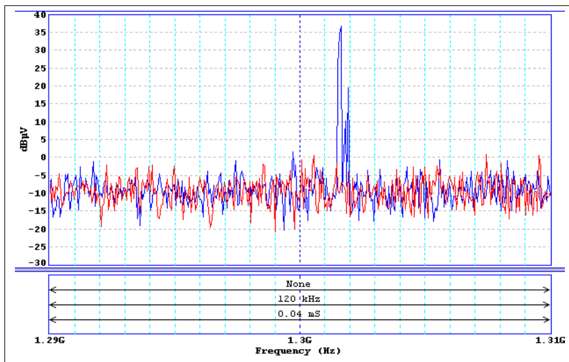
Fig.3. Third harmonic emission spectrum of the EUT. Blue is with the EUT functioning and Red is the ambient. The field was measured with an EMCO 3143 broadband vertically polarized antenna located 3-m from the EUT.
