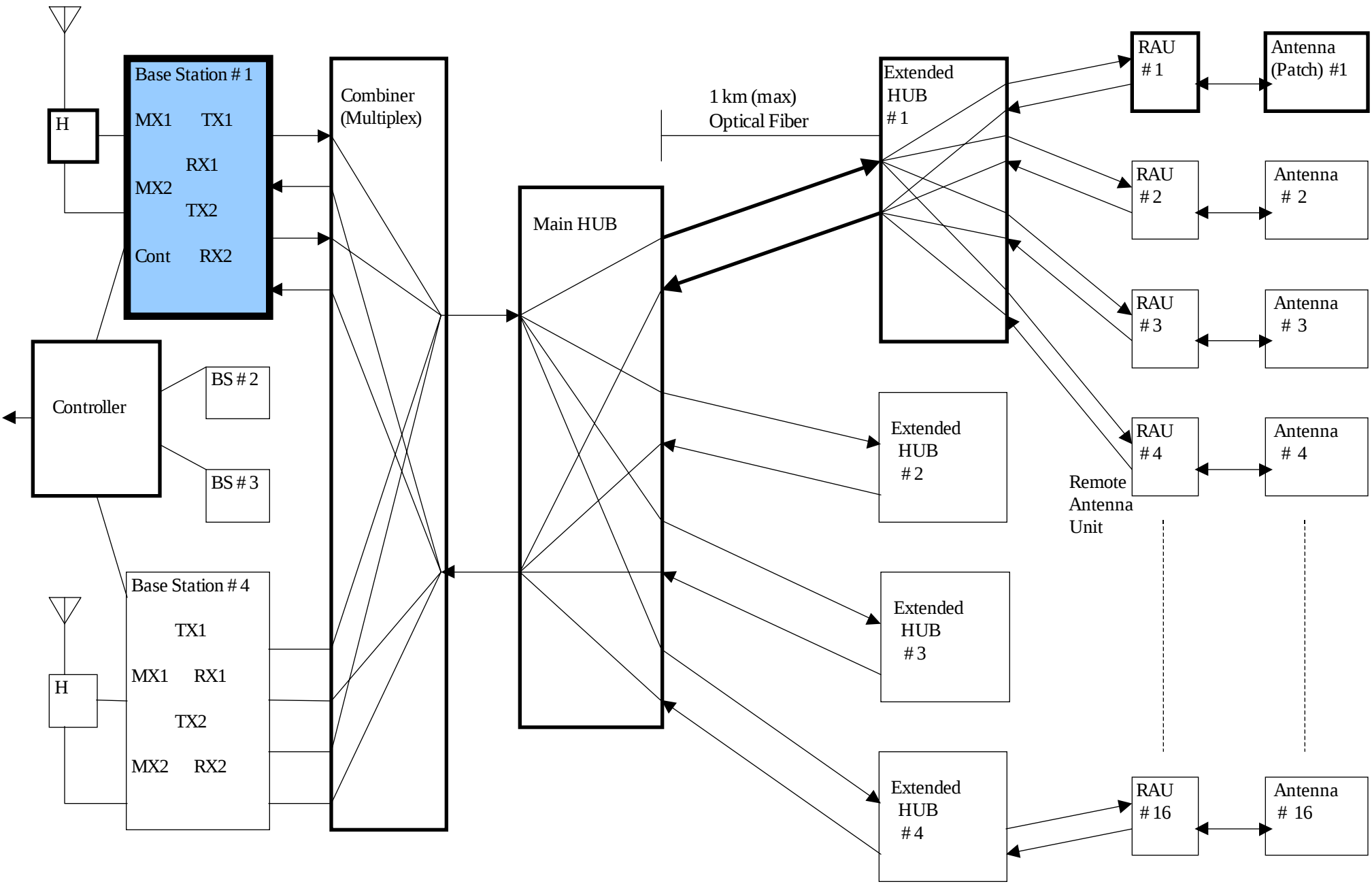
General Configuration of Base Stations and Distributed Antenna System
