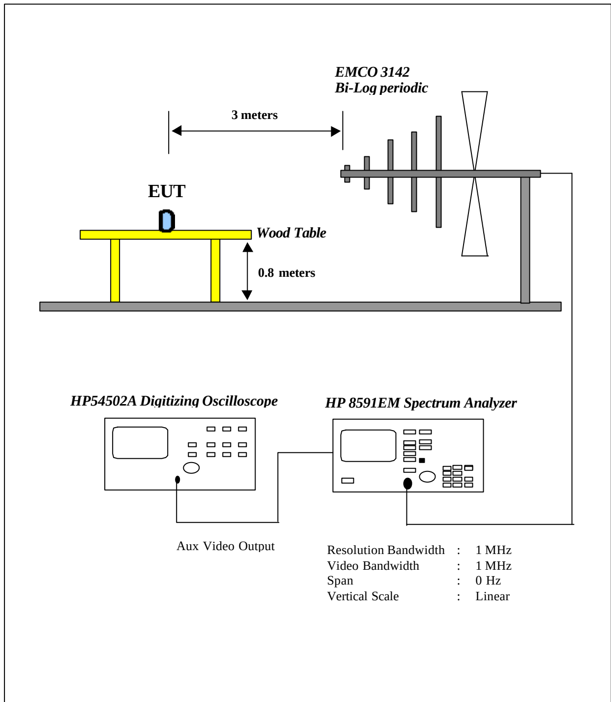
fig 1. Test Configuration of Duty Cycle Measurement
