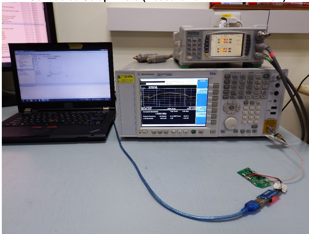
Conducted Setup Photo (Measurement at Antenna Port)
