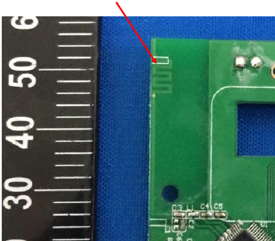
PCB Antenna – View
