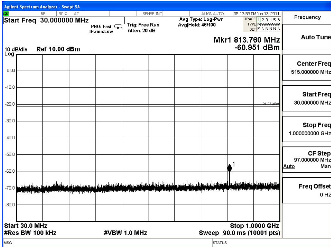
Figure Channel 39: 30M-1GHz
