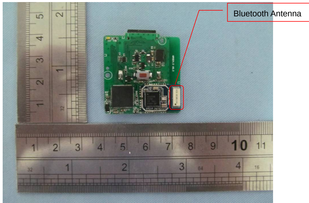
Front View of PCB
