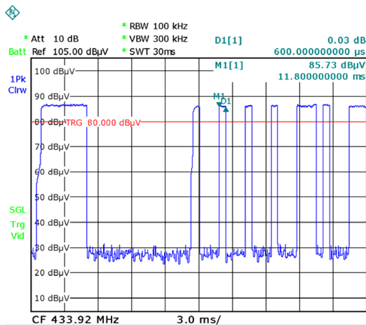
Pulse 2
