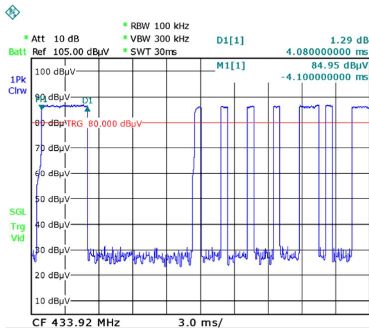
Pulse 1
