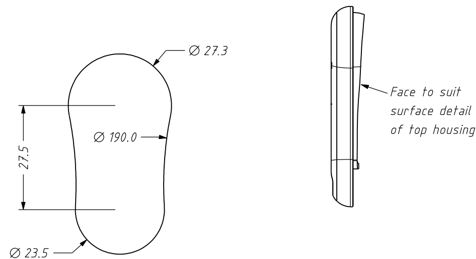
EXTERNAL PROFILE
