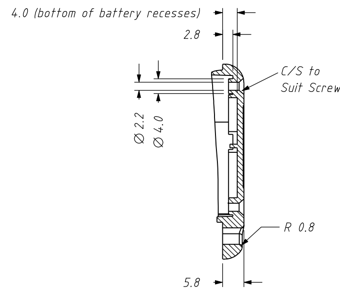
SECTION THRU' Q-Q
