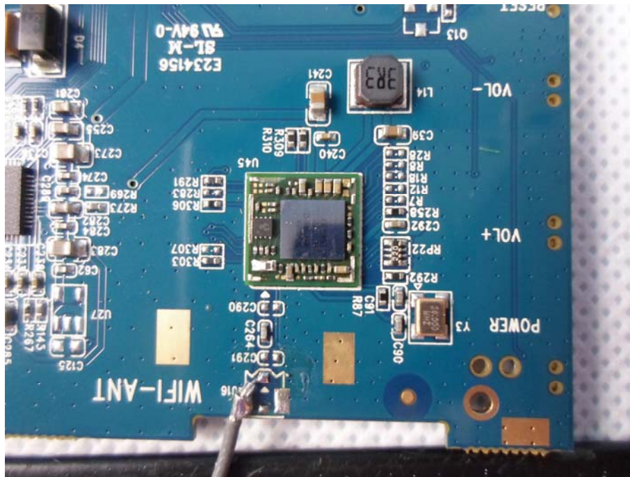
Photo 12 WiFi Module
