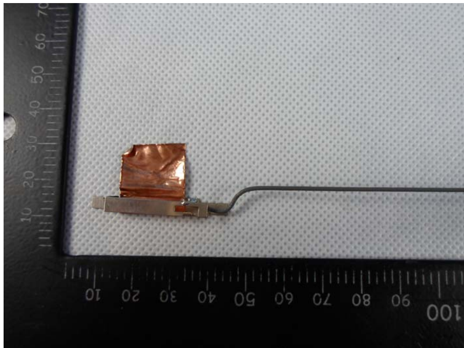
Photo 13 Antenna
