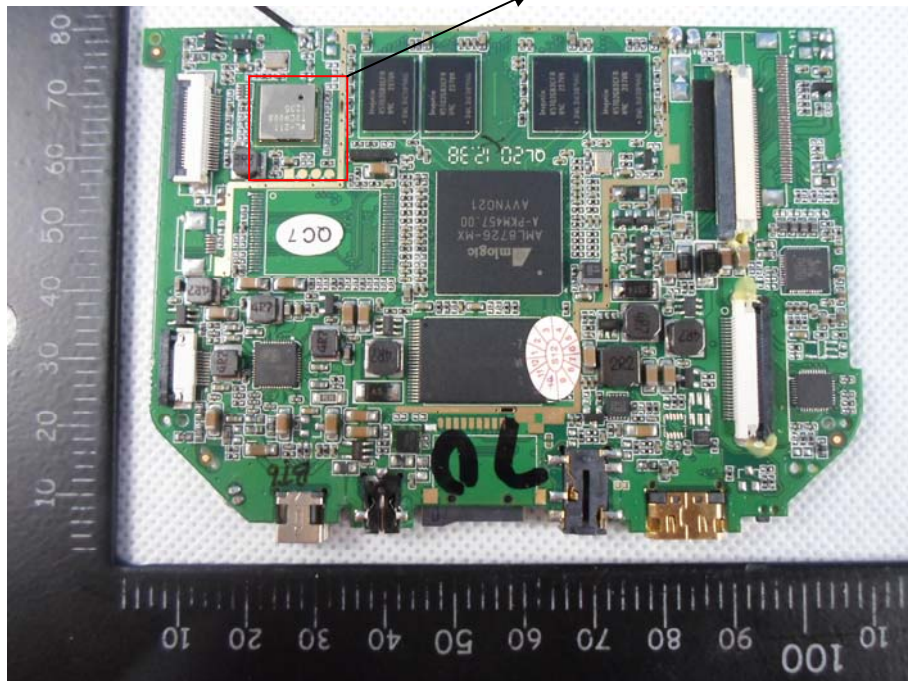
Photo 9 WiFi Module
