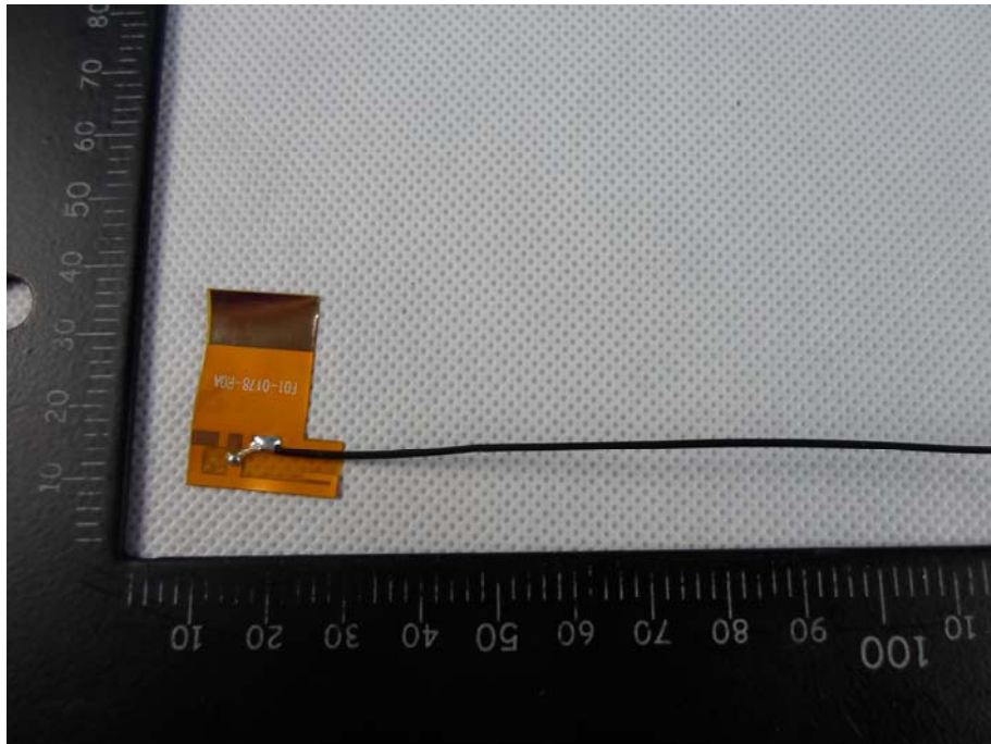
Photo 15 WiFi Antenna
