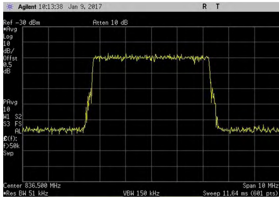
7.10_OBW_UL_824-849MHz_LTE_In
