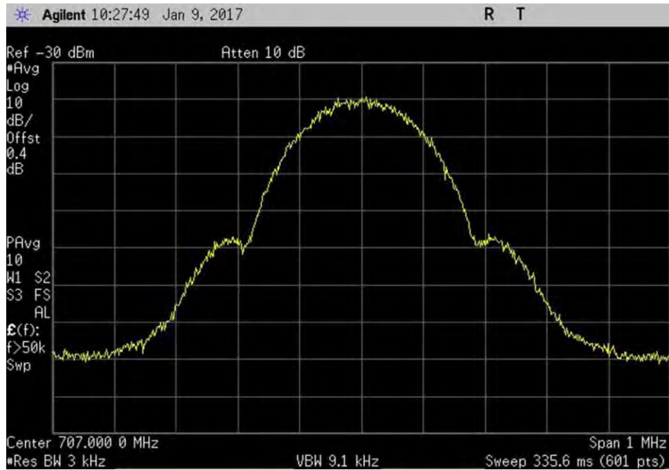
7.10_OBW_UL_698-716MHz_GSM_In
