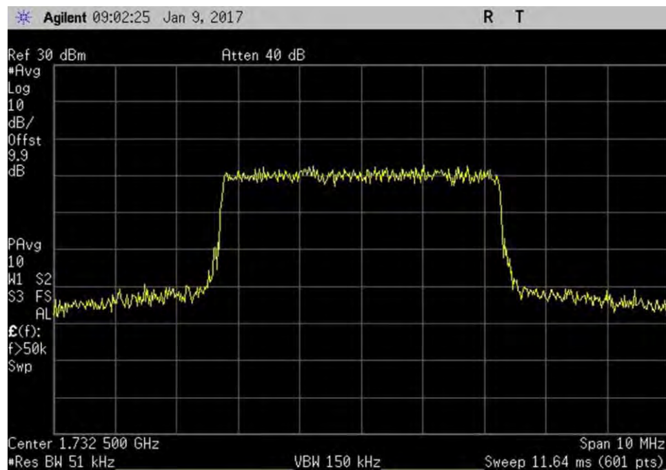
7.10_OBW_UL_1710-1755MHz_LTE_Out
