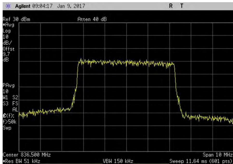
7.10_OBW_UL_824-849MHz_LTE_Out
