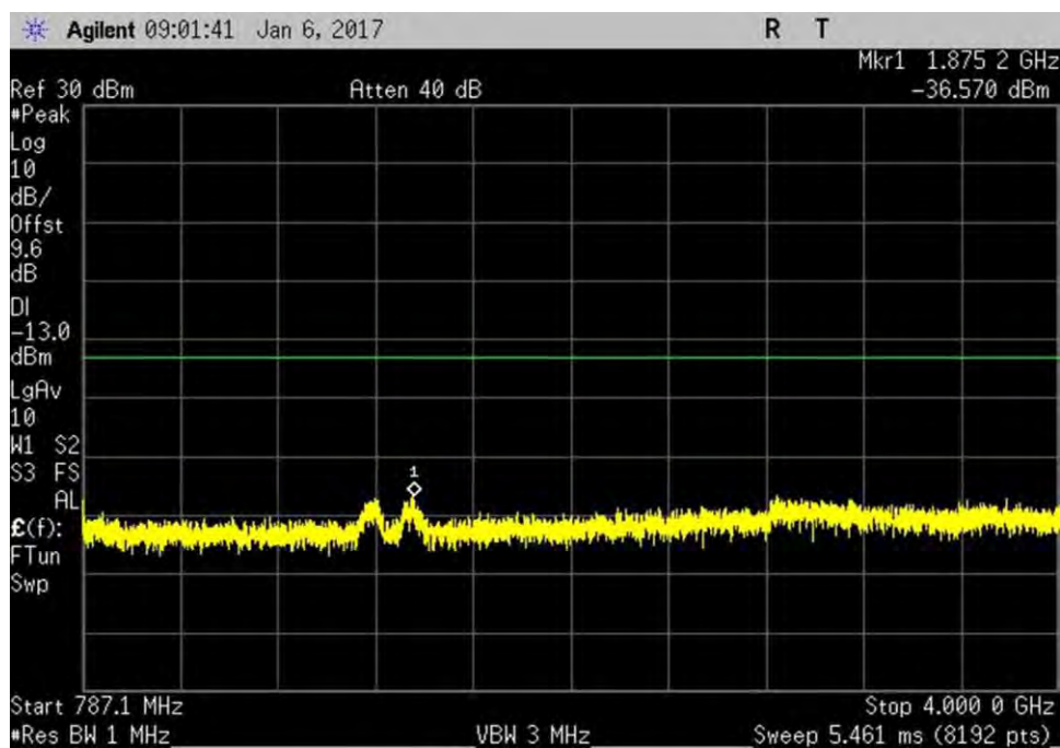
7.6_CSE_UL_776-787MHz_R1
