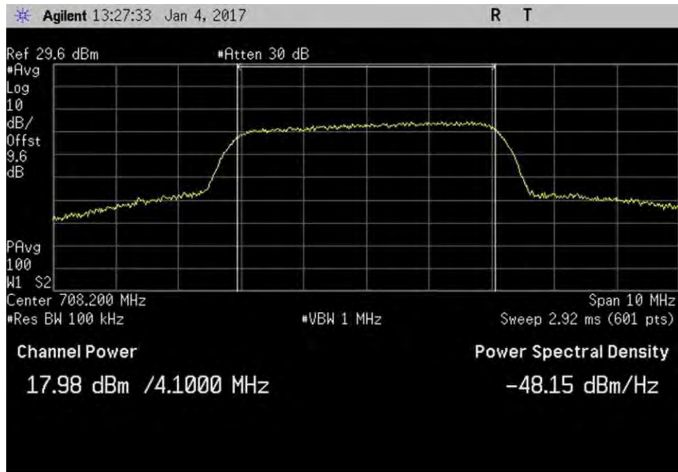
7.2_Power_UL_698-716MHz_AWGN
