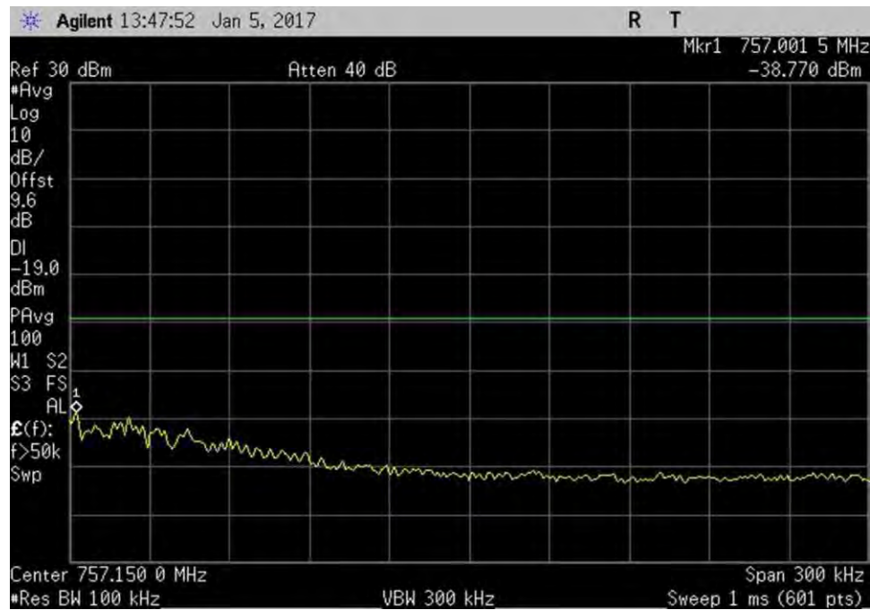
7.5_OBE_DL_746-757MHz_H_PreAGC_LTE
