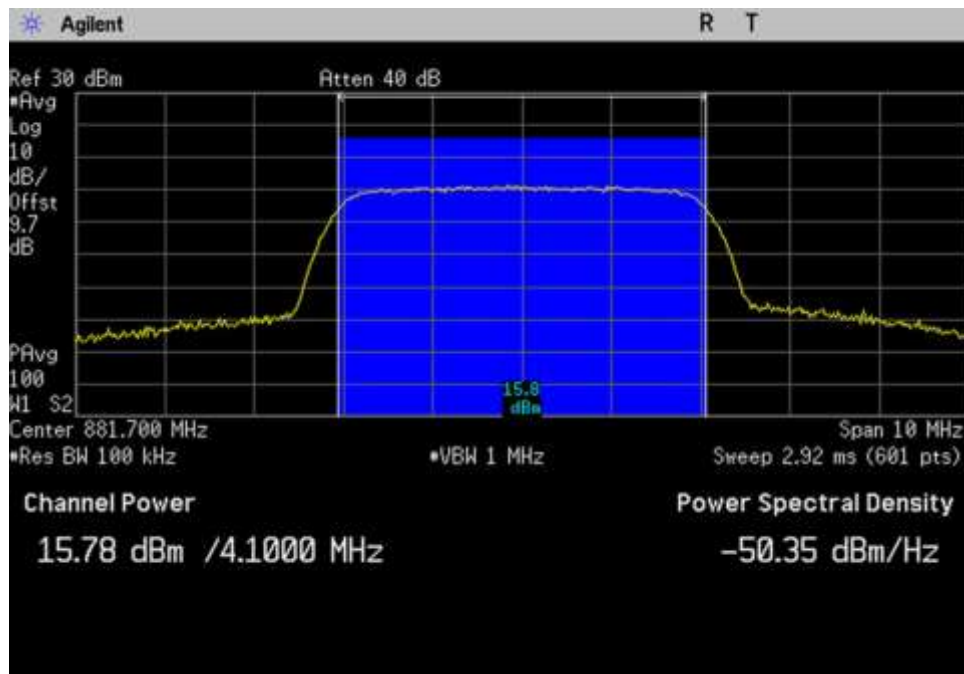
DL_869-894MHz_AWGN
