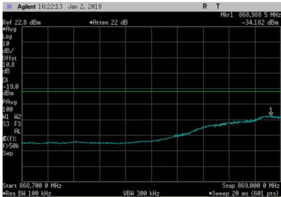
DL_ 868.7- 869MHz_LTE
