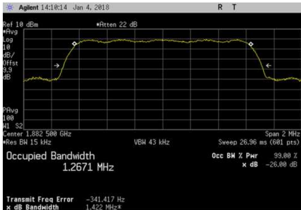
UL_ 1882.5MHz_CDMA
