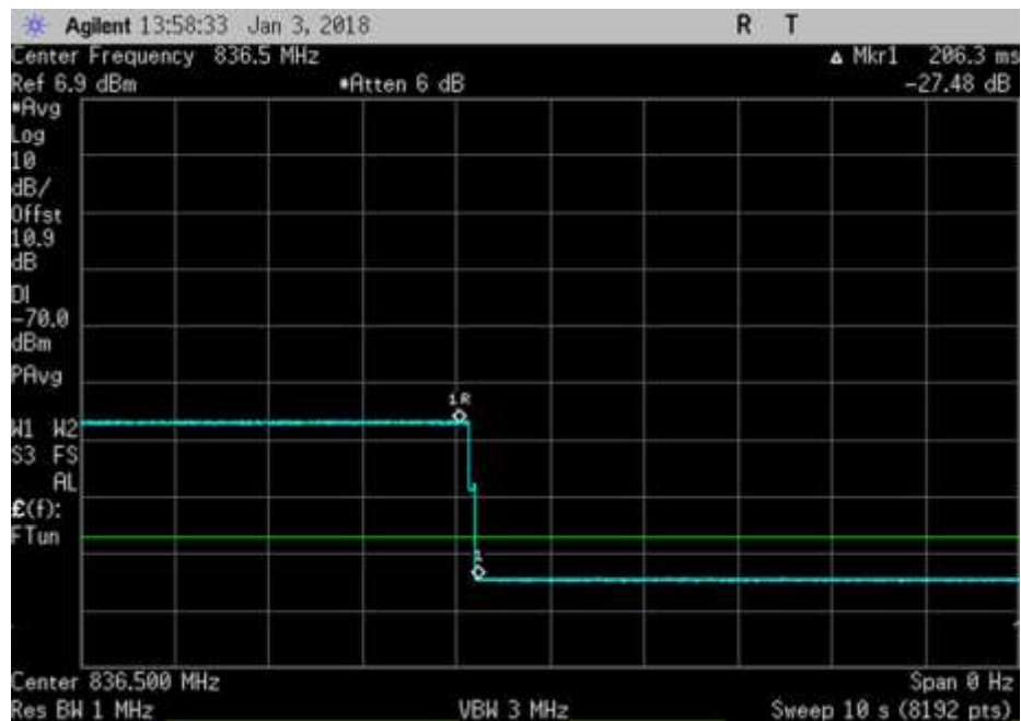
UL_836.5MHz_time
