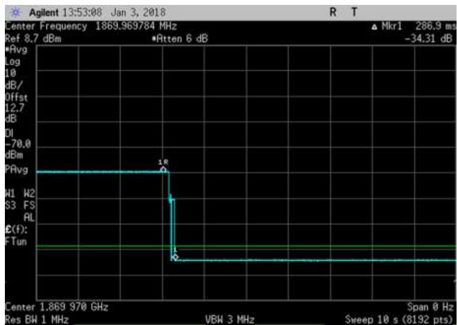
UL_1869.969784MHz_time
