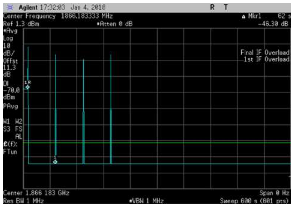
UL_ 1866.183333MHz_600sec
