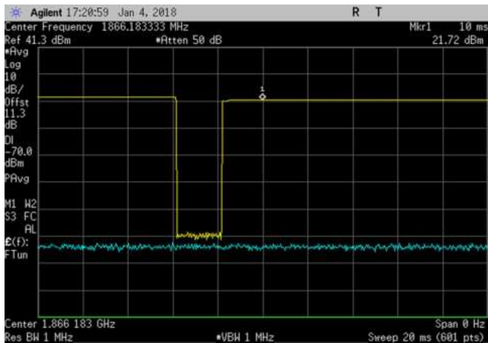
UL_ 1866.183333MHz_Peak
