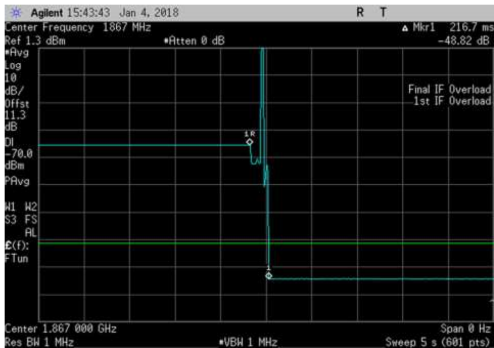
UL_ 1867MHz_Mitigation time
