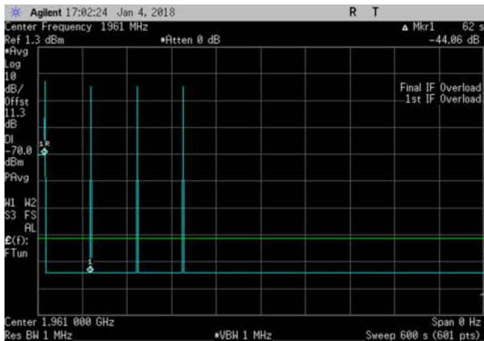
DL_1961MHz_600sec
