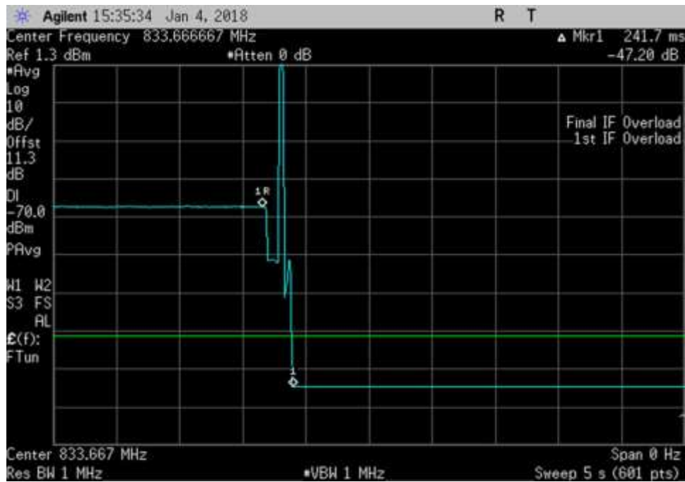
UL_ 833.6MHz_Mitigation time
