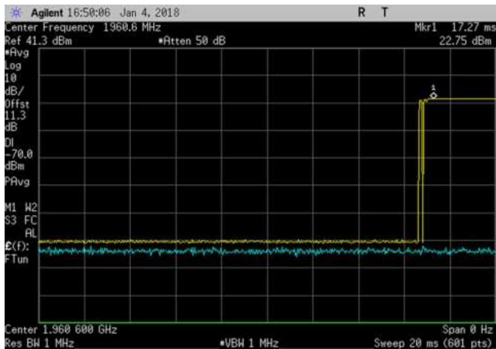
DL_1960.6MHz_Peak
