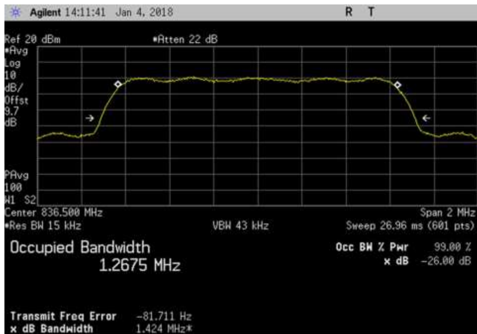
UL_ 836.5MHz_CDMA
