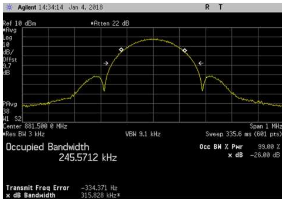
DL_881.5MHz_EDGE
