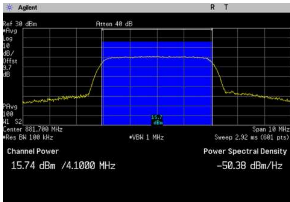
DL_869-894MHz_AWGN_Max
