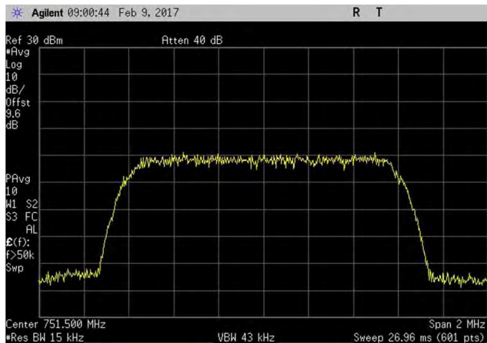
7.10_OBW_DL_746-757MHz_CDMA_Out
