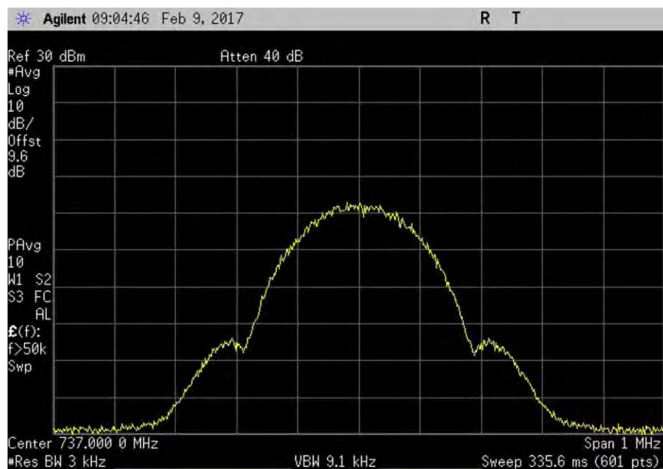
7.10_OBW_DL_728-746MHz_GSM_Out
