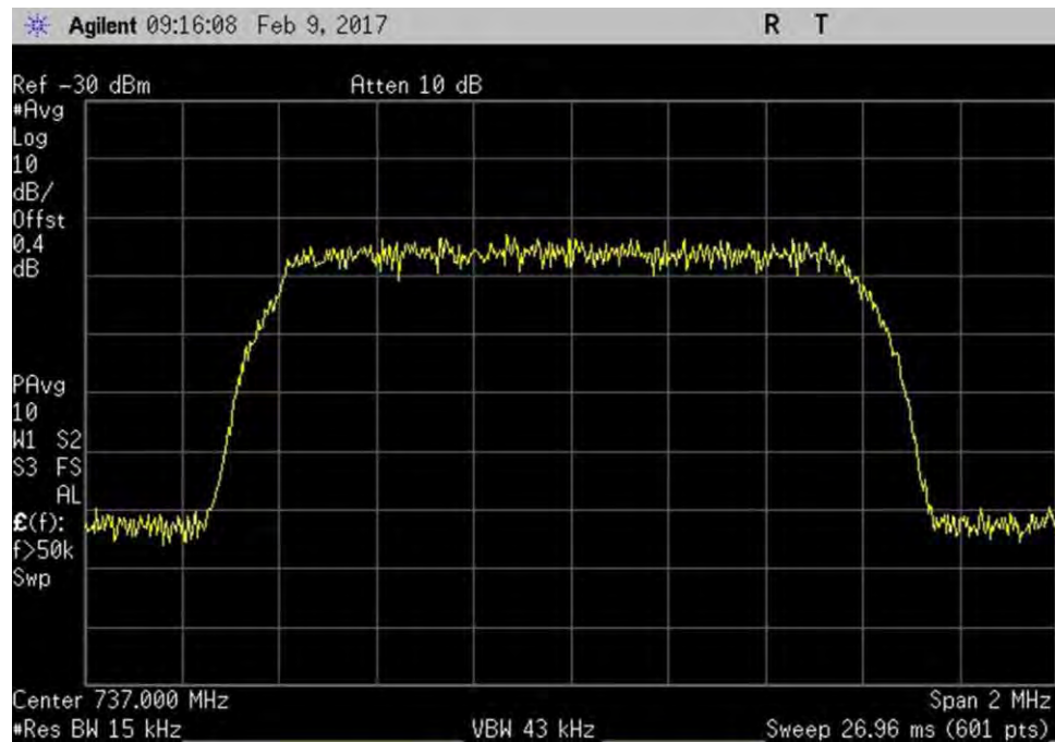
7.10_OBW_DL_728-746MHz_CDMA_In
