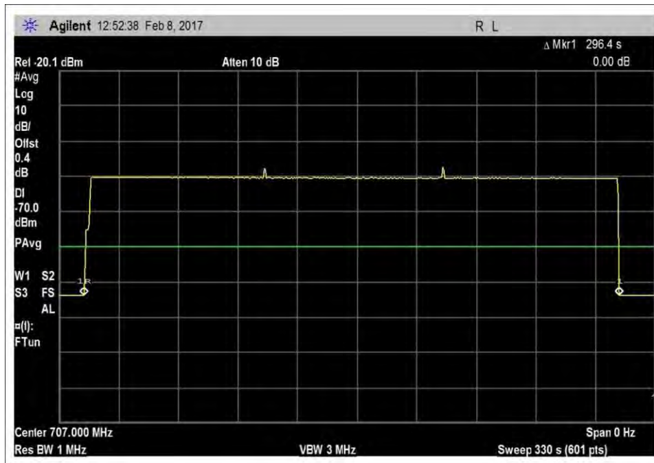
7.8_InactivityUL_698-716MHz
