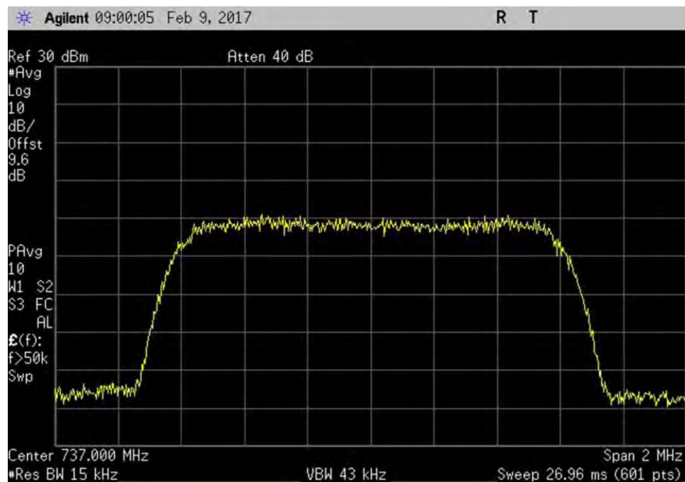
7.10_OBW_DL_728-746MHz_CDMA_Out
