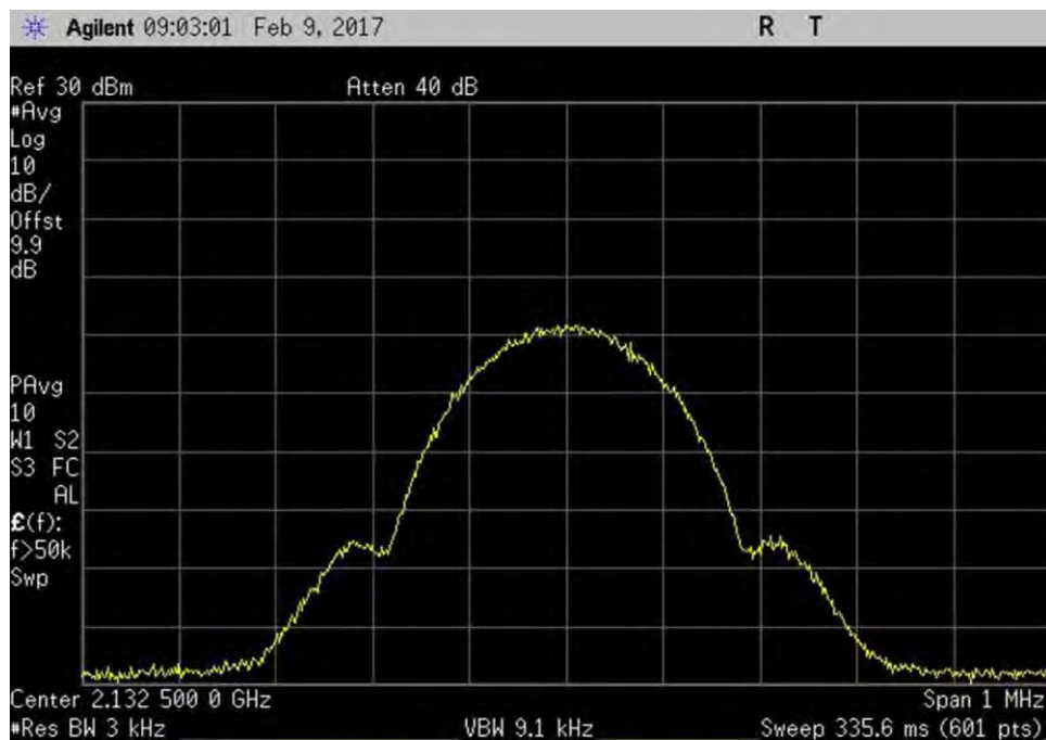
7.10_OBW_DL_2110-2155MHz_GSM_Out
