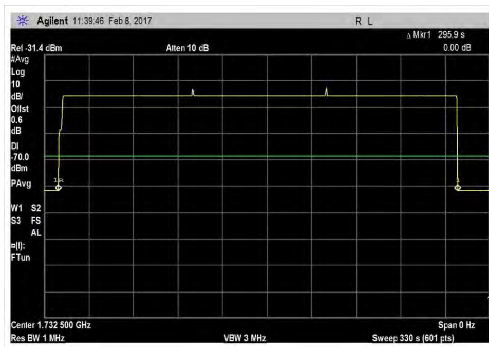
7.8_Inactivity_UL_1710-1755MHz
