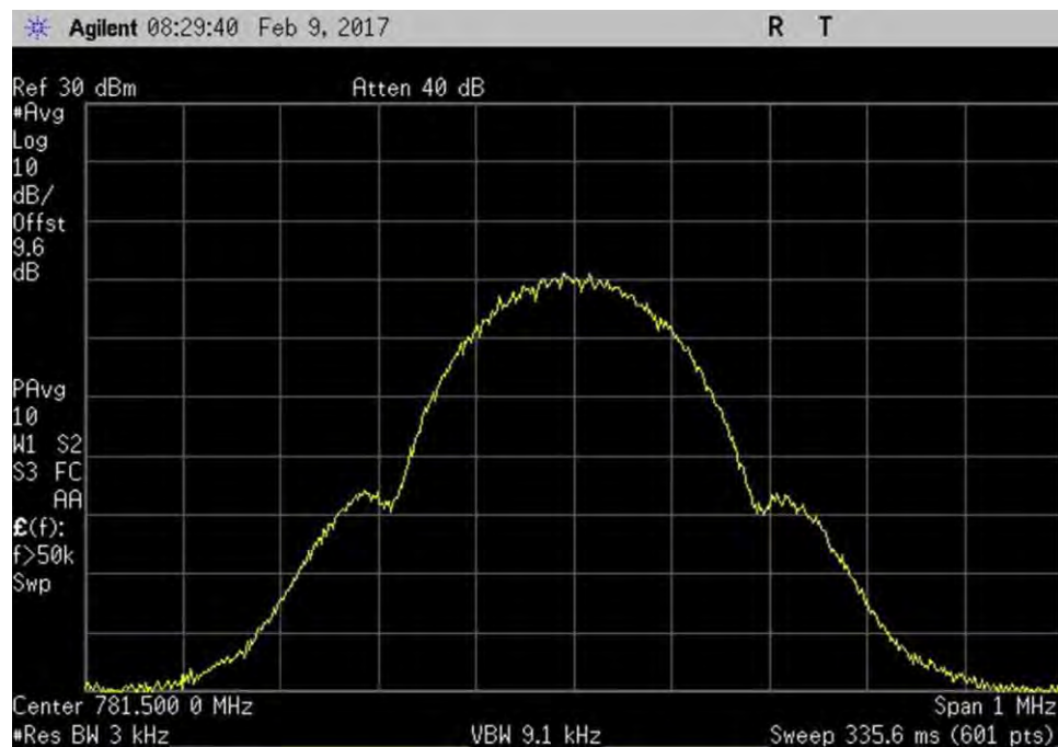
7.10_OBW_UL_776-787MHz_GSM_Out
