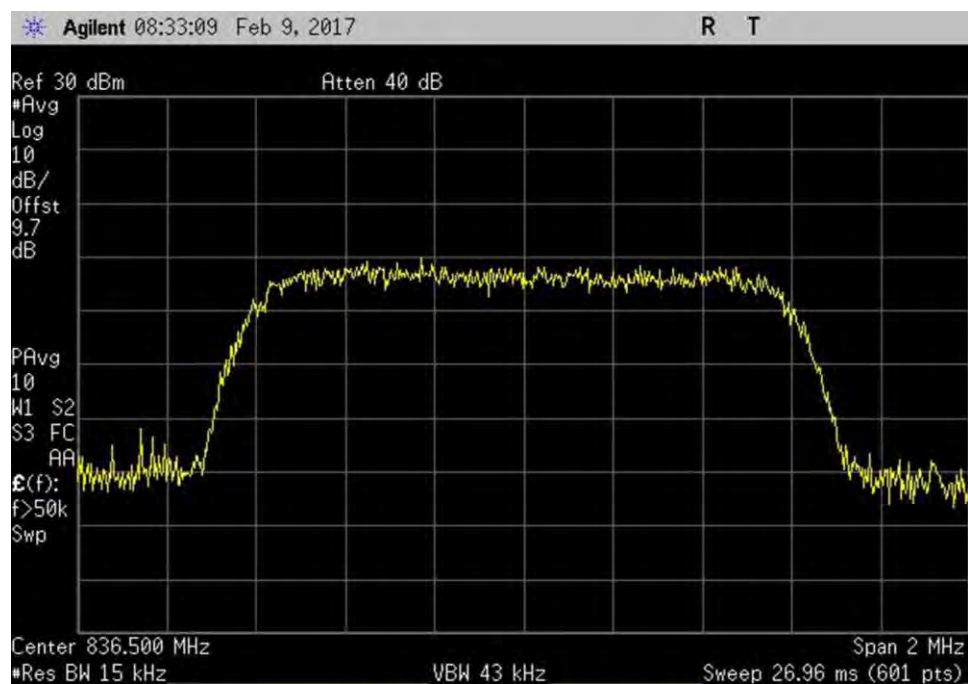
7.10_OBW_UL_824-849MHz_CDMA_Out
