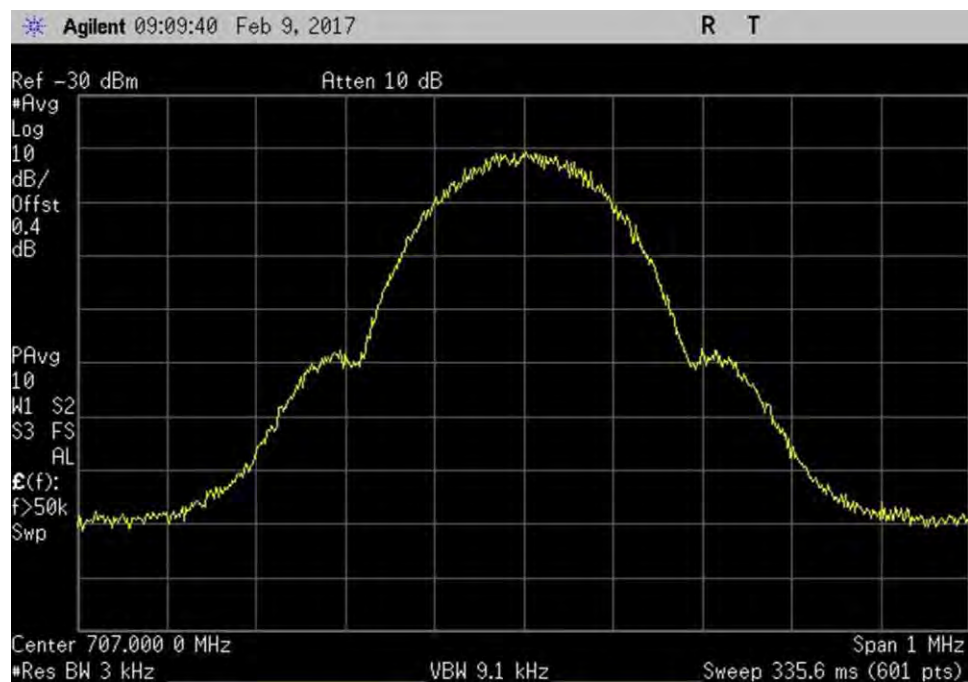
7.10_OBW_UL_698-716MHz_GSM_In
