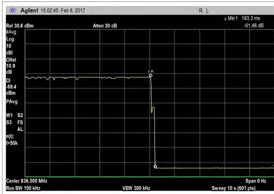
7.9.2_VarULGainTiming_UL_824-849MHz
