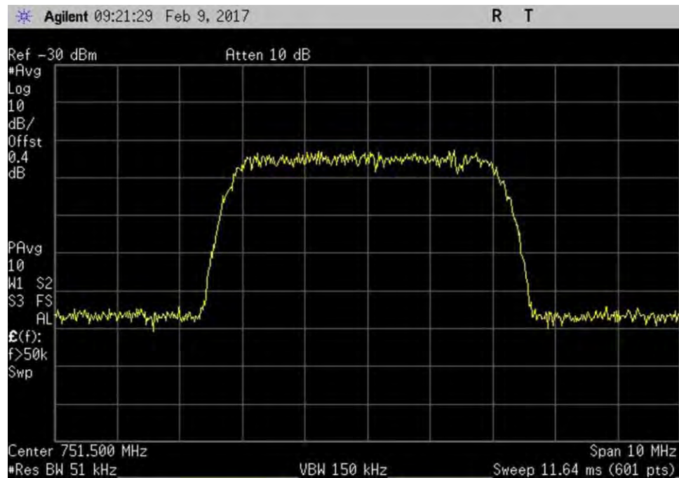
7.10_OBW_DL_746-757MHz_WCDMA_In
