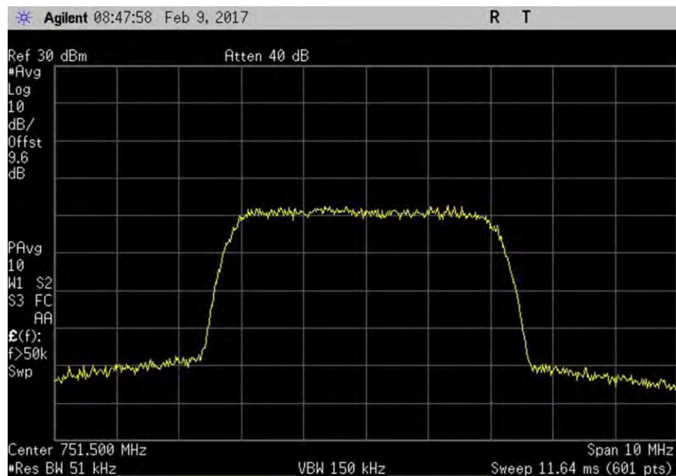
7.10_OBW_DL_746-757MHz_WCDMA_Out
