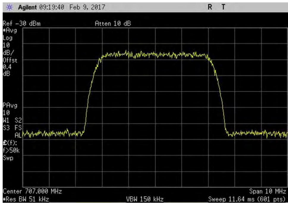
7.10_OBW_UL_698-716MHz_WCDMA_In
