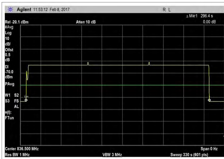
7.8_InactivityUL_824-849MHz
