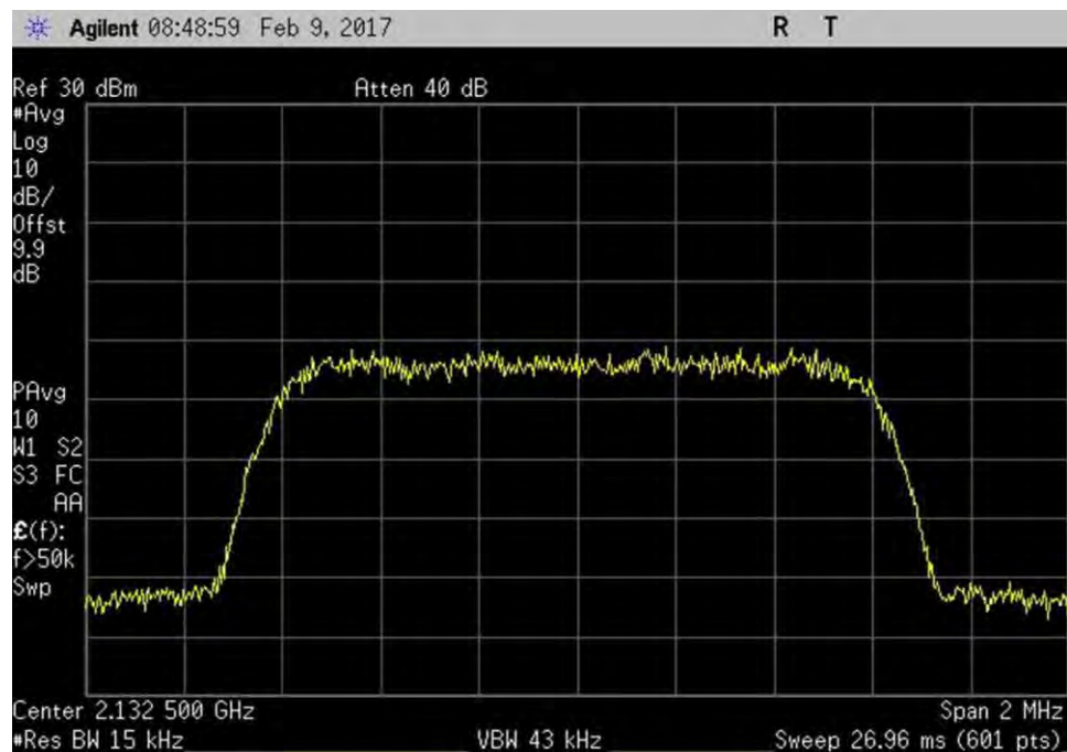
7.10_OBW_DL_2110-2155MHz_CDMA_Out
