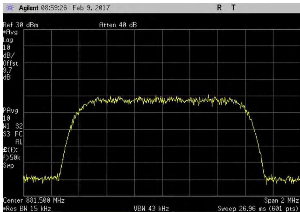
7.10_OBW_DL_869-894MHz_CDMA_Out
