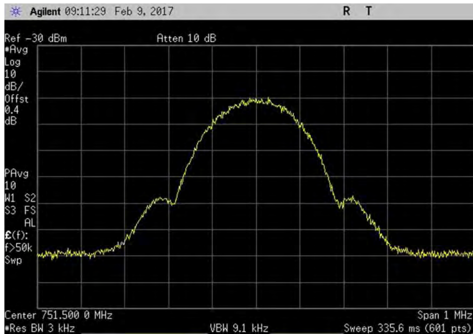
7.10_OBW_DL_746-757MHz_GSM_In
