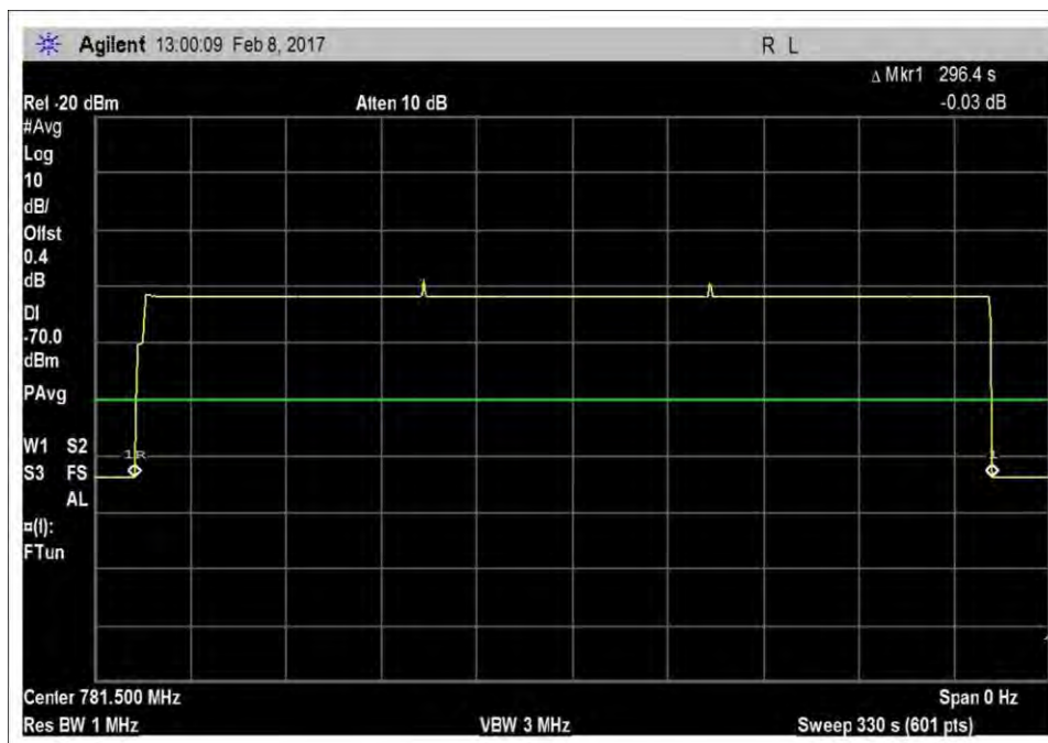
7.8_InactivityUL_776-787MHz
