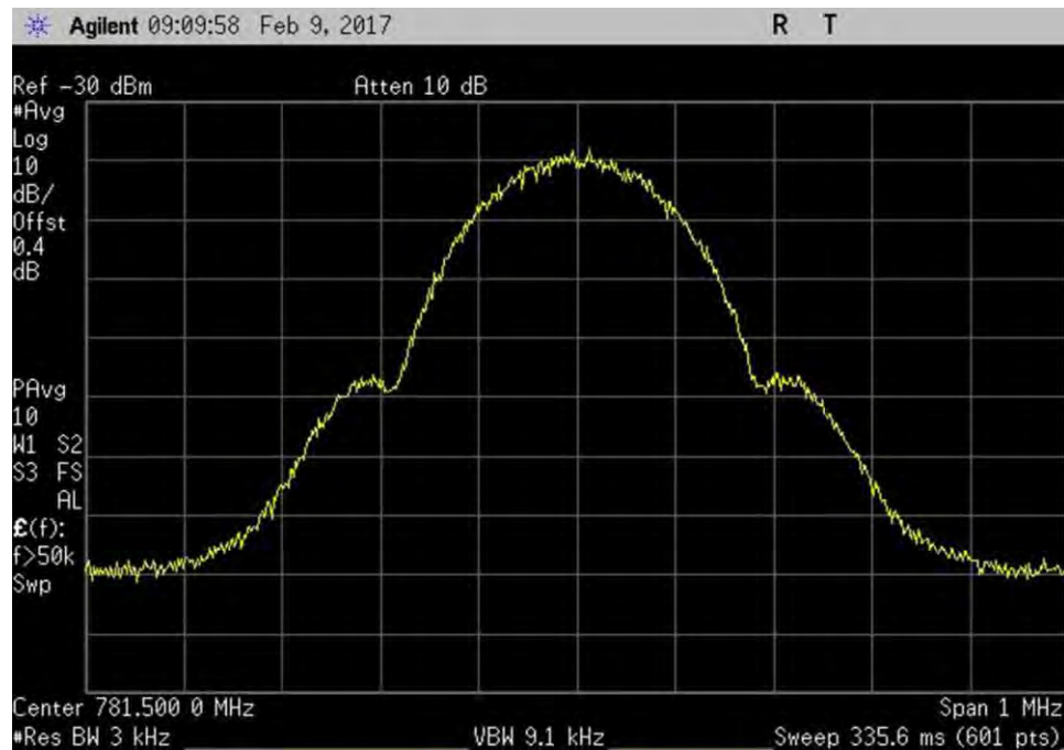
7.10_OBW_UL_776-787MHz_GSM_In
