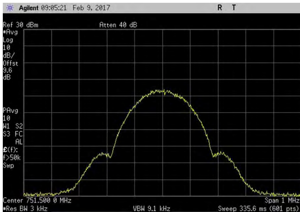
7.10_OBW_DL_746-757MHz_GSM_Out
