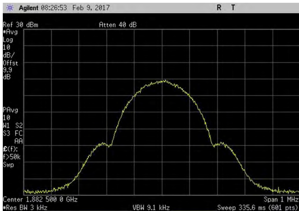
7.10_OBW_UL_1850-1915MHz_GSM_Out
