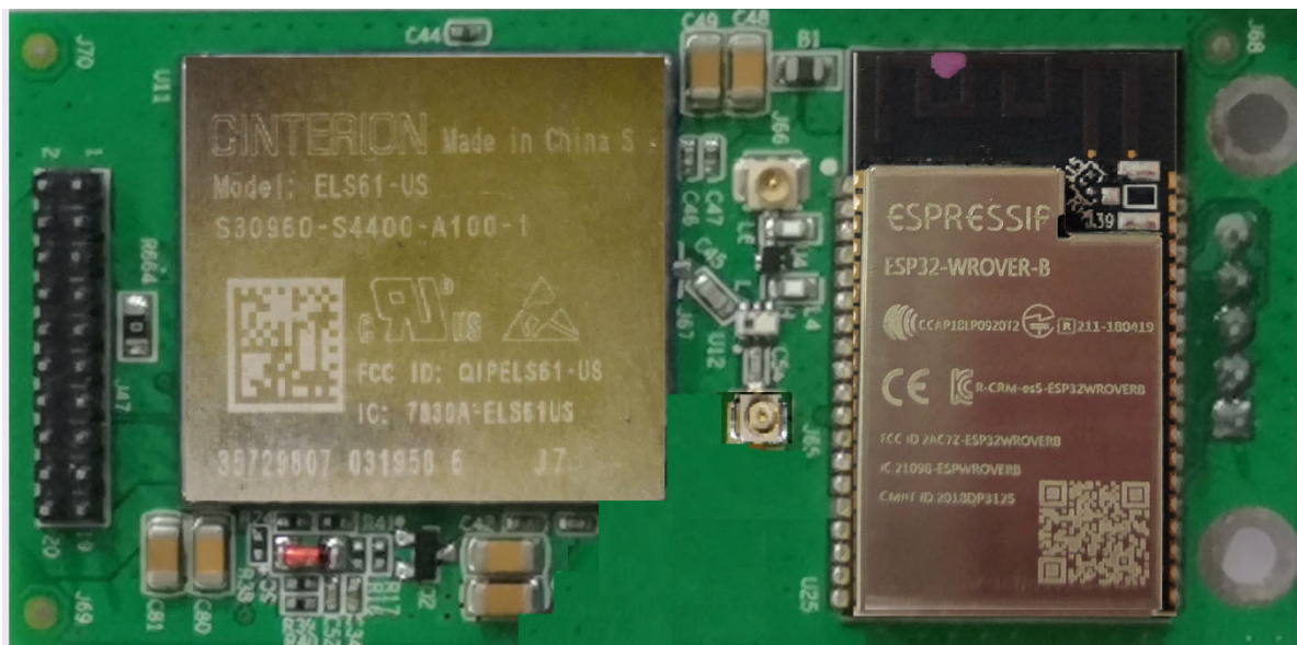
EUT – Mainboard 5 Top View
