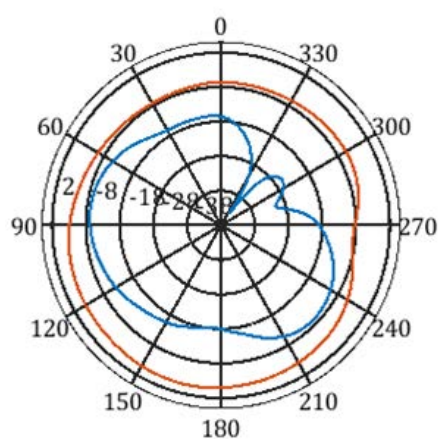
f=1710MHz,X-Y Plane
