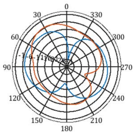
f=960MHz,X-Y Plane
