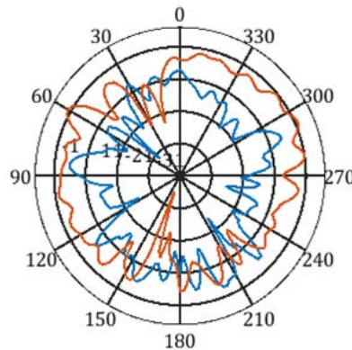
f=1710MHz,@Y-Z plane
