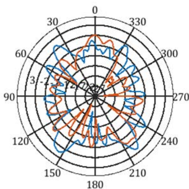
f=960MHz,@Y-Z plane
