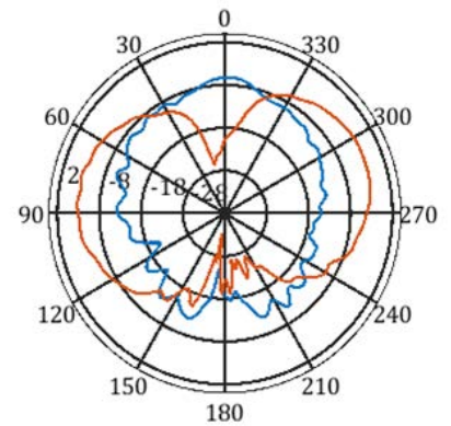
f=2500MHz,@Y-Z plane
