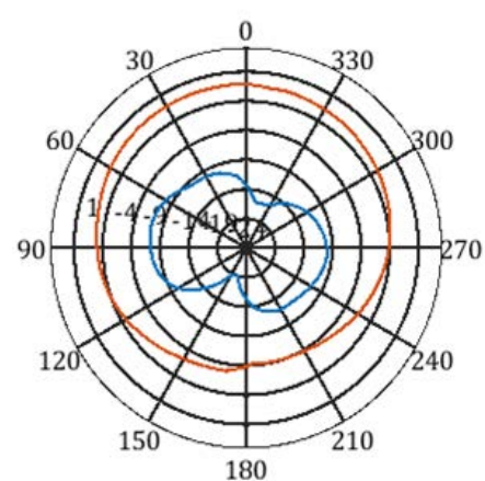
f=2500MHz,X-Y Plane
