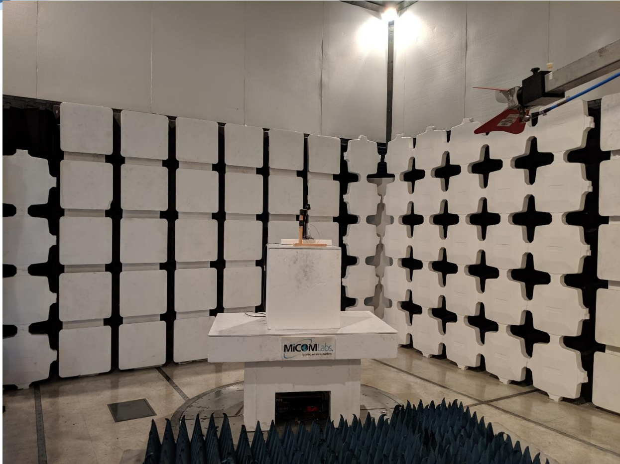
Radiated Spurious Emissions 1-12.75GHz
