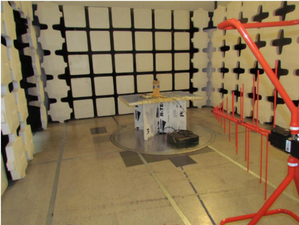
External Antenna
