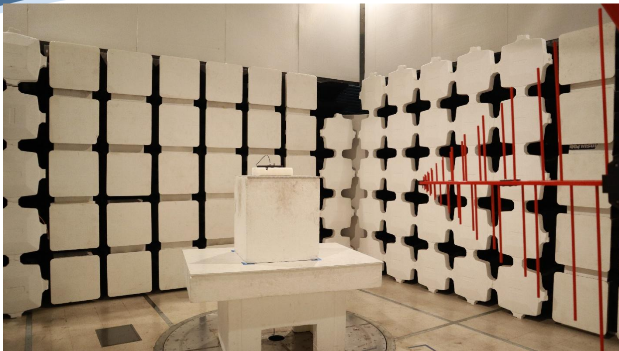
Radiated Emissions 30M-1GHz
