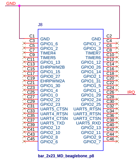
bar_2x23_MD_beaglebone_p8
