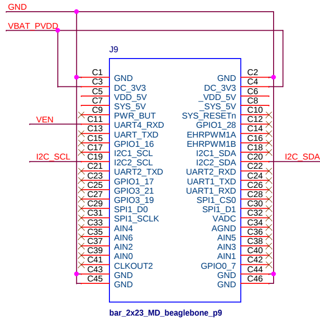
bar_2x23_MD_beaglebone_p9
