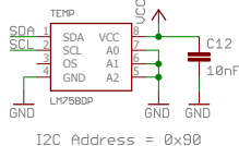
LM75B I2C TEMPERATURE SENSOR
