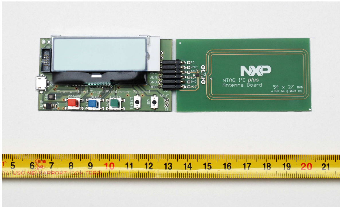
Picture 1: NTAG I 2 C plus Explorer Kit - top view.
