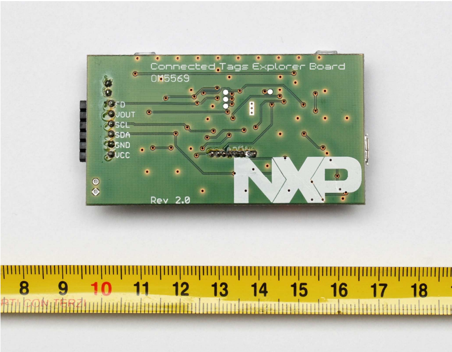
Picture 4: Connected Tags Explorer Board – bottom view.
