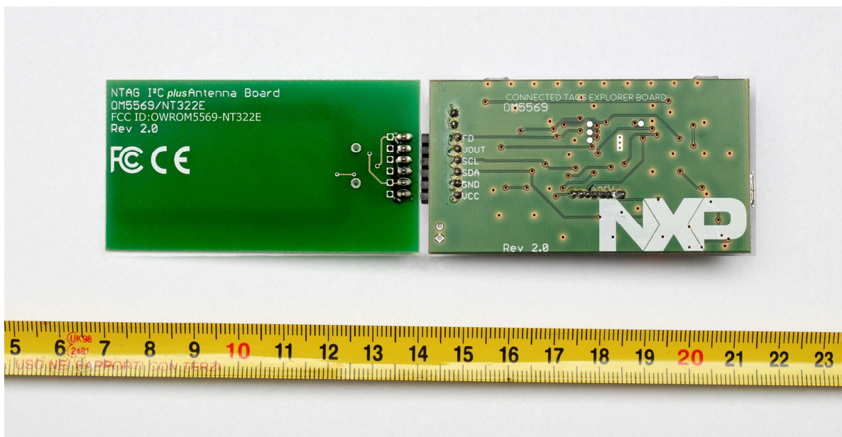
Picture 2: NTAG I 2 C plus Explorer Kit - bottom view.
