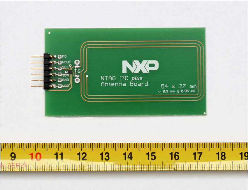
Picture 5: NTAG I 2 C plus Antenna Board 54 x 27 mm – top view.
