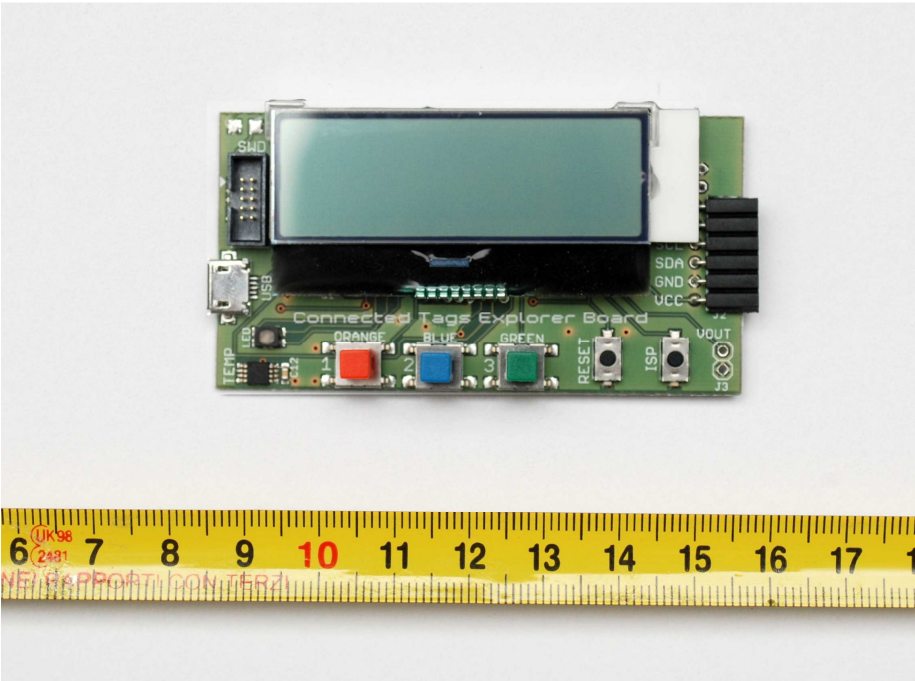
Picture 3: Connected Tags Explorer Board – top view.
