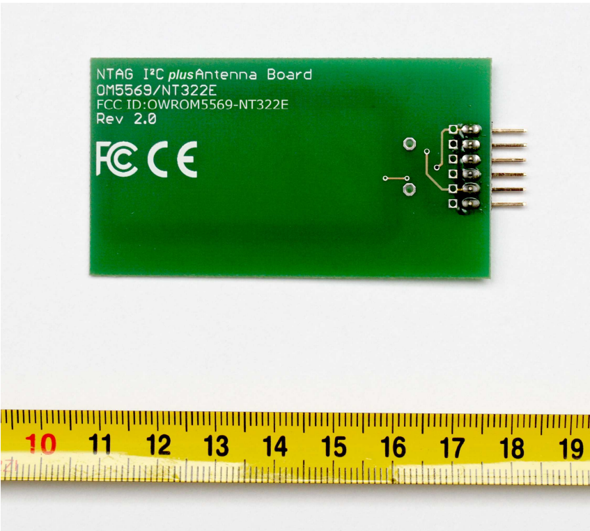
Picture 6: NTAG I 2 C plus Antenna Board 54 x 27 mm – bottom view.
