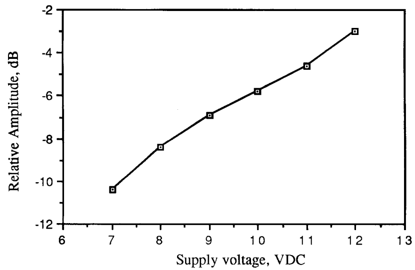
Figure 6.4. Relative emission at 310.0 MHz vs. supply voltage. (pulsed emission)
