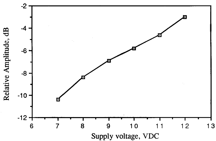
Figure 6.4. Relative emission at 300.0 MHz vs. supply voltage. (pulsed emission)
