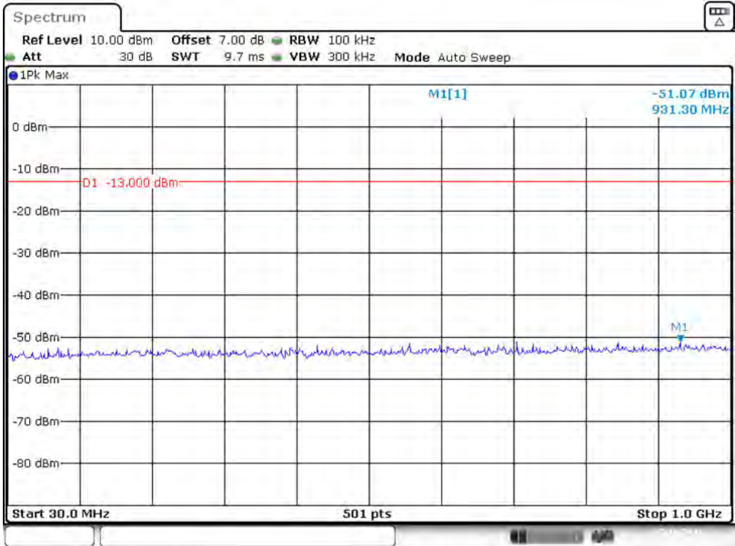
Band 4_3 MHz_High_QPSK_RB15#0_1(30MHz-1GHz)
