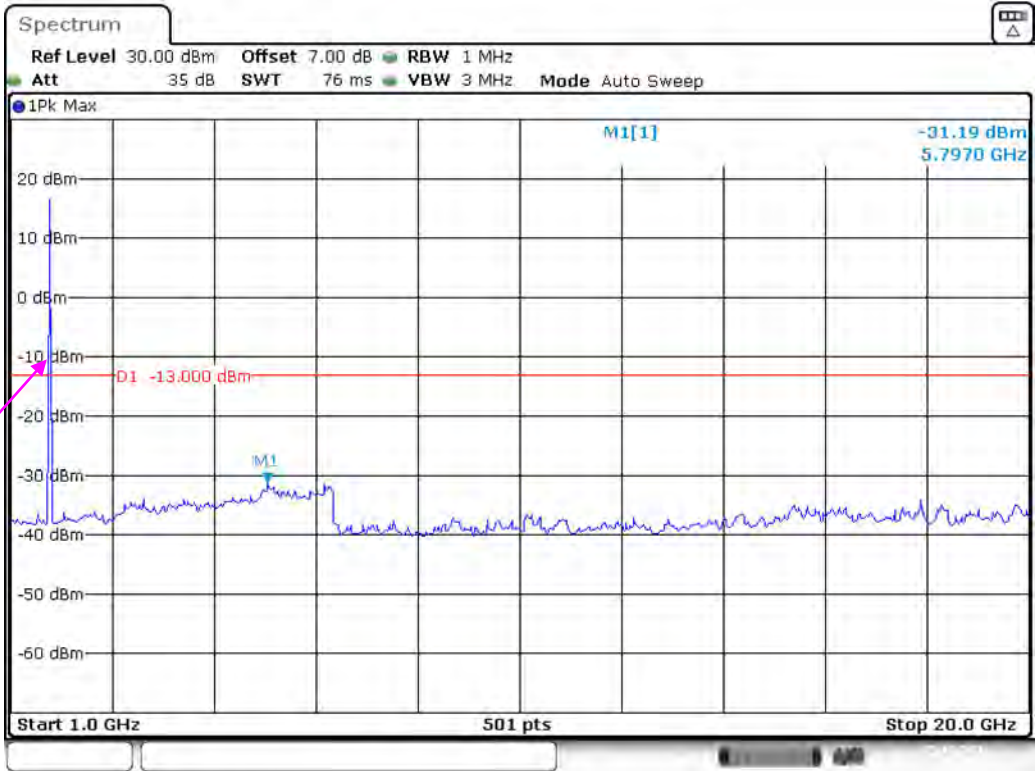
Band 4_20 MHz_High_QPSK_RB100#0_2(1GHz-20GHz)
