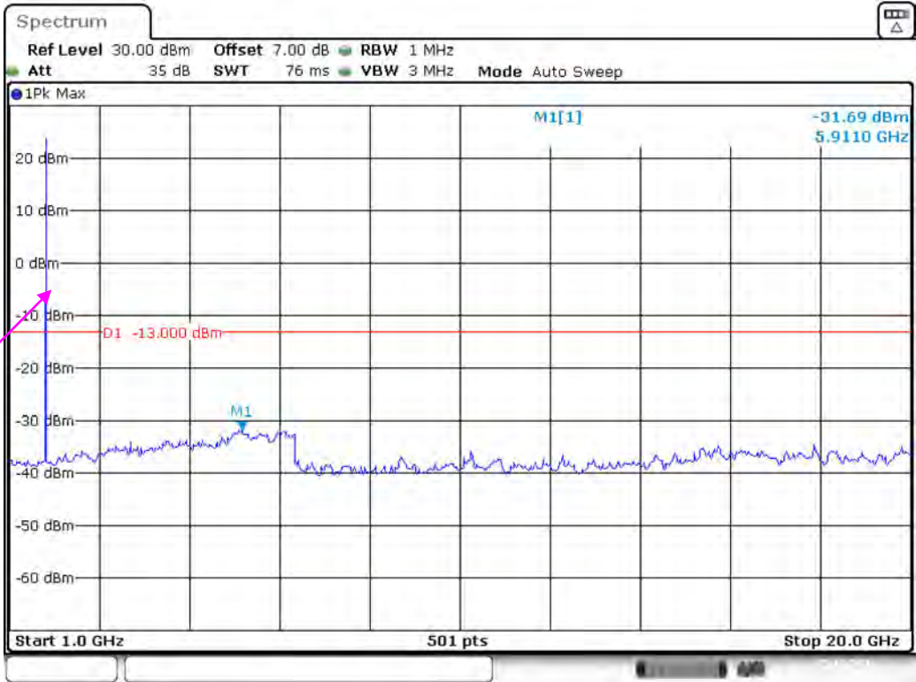
Band 66_1.4 MHz_High_QPSK_RB6#0_2(1GHz-20GHz)
