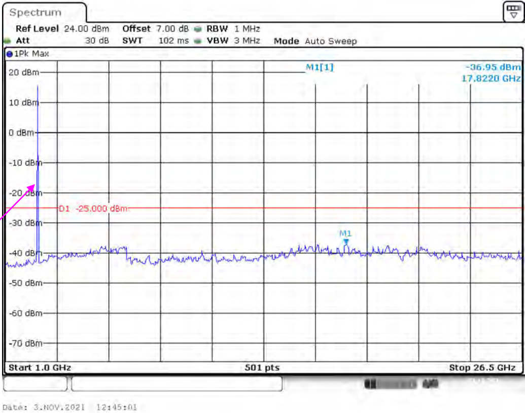
Band 38_10 MHz_High_QPSK_RB50#0_2(1GHz-26.5GHz)
