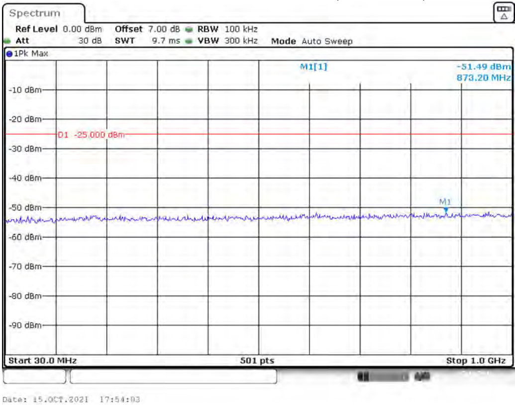
Band 7_15 MHz_Low_QPSK_RB75#0_1(30MHz-1GHz)
