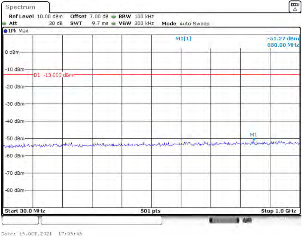
Band 2_3 MHz_Low_QPSK_RB15#0_1(30MHz-1GHz)
