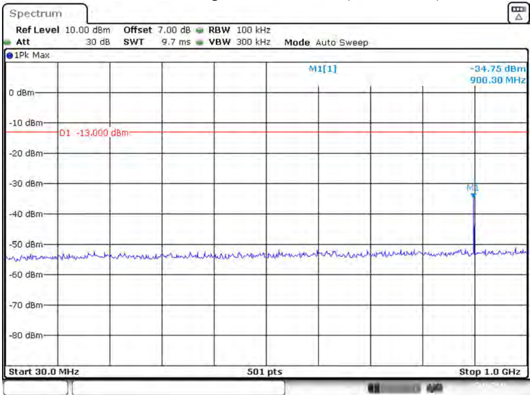
Band 66_3 MHz_High_QPSK_RB15#0_1(30MHz-1GHz)
