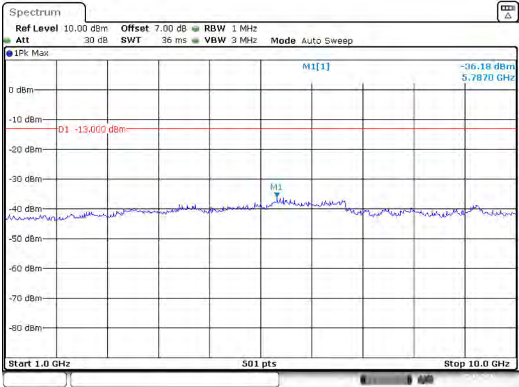
Band 5_5 MHz_High_QPSK_RB25#0_2(1GHz-10GHz)
