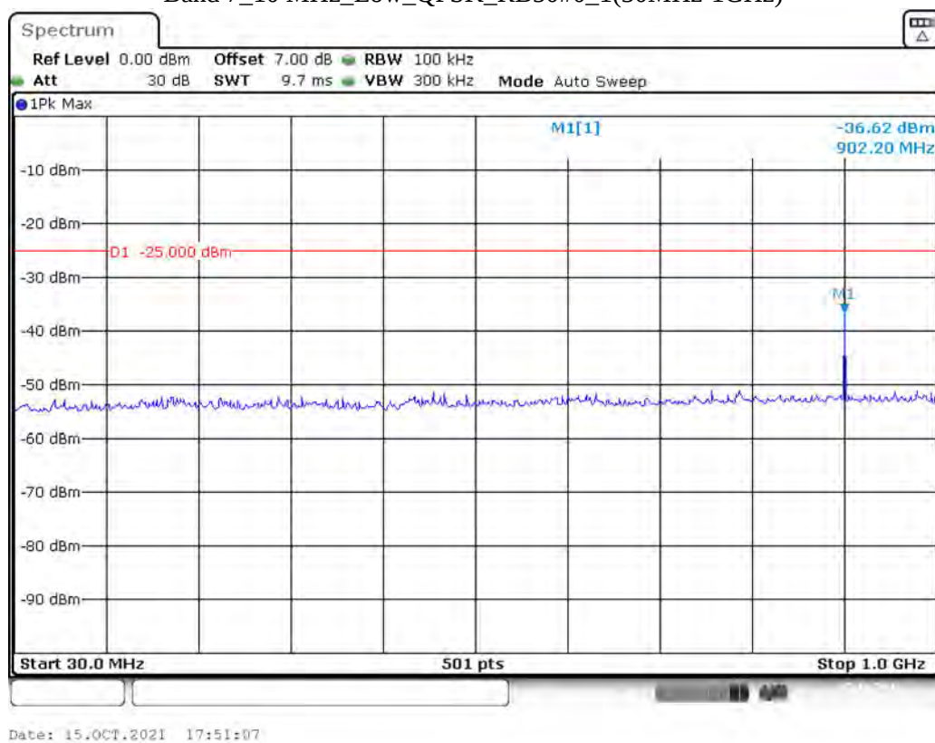
Band 7_10 MHz_Low_QPSK_RB50#0_1(30MHz-1GHz)
