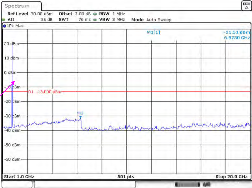
Band 66_3 MHz_Middle_QPSK_RB15#0_2(1GHz-20GHz)
