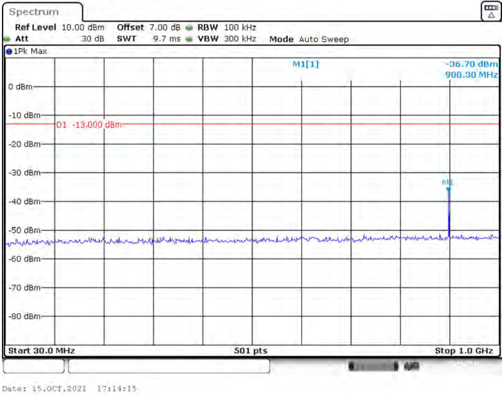
Band 2_15 MHz_Low_QPSK_RB75#0_1(30MHz-1GHz)
