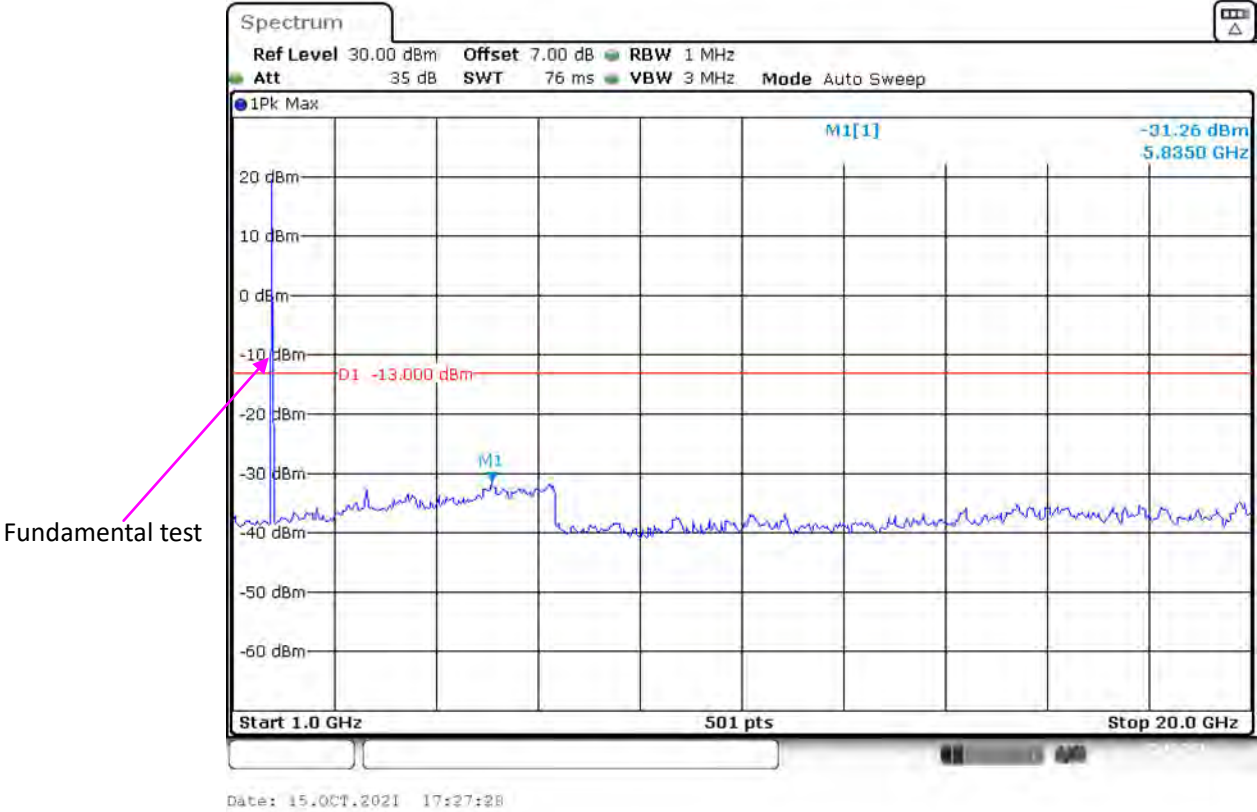
Band 4_5 MHz_High_QPSK_RB25#0_2(1GHz-20GHz)
