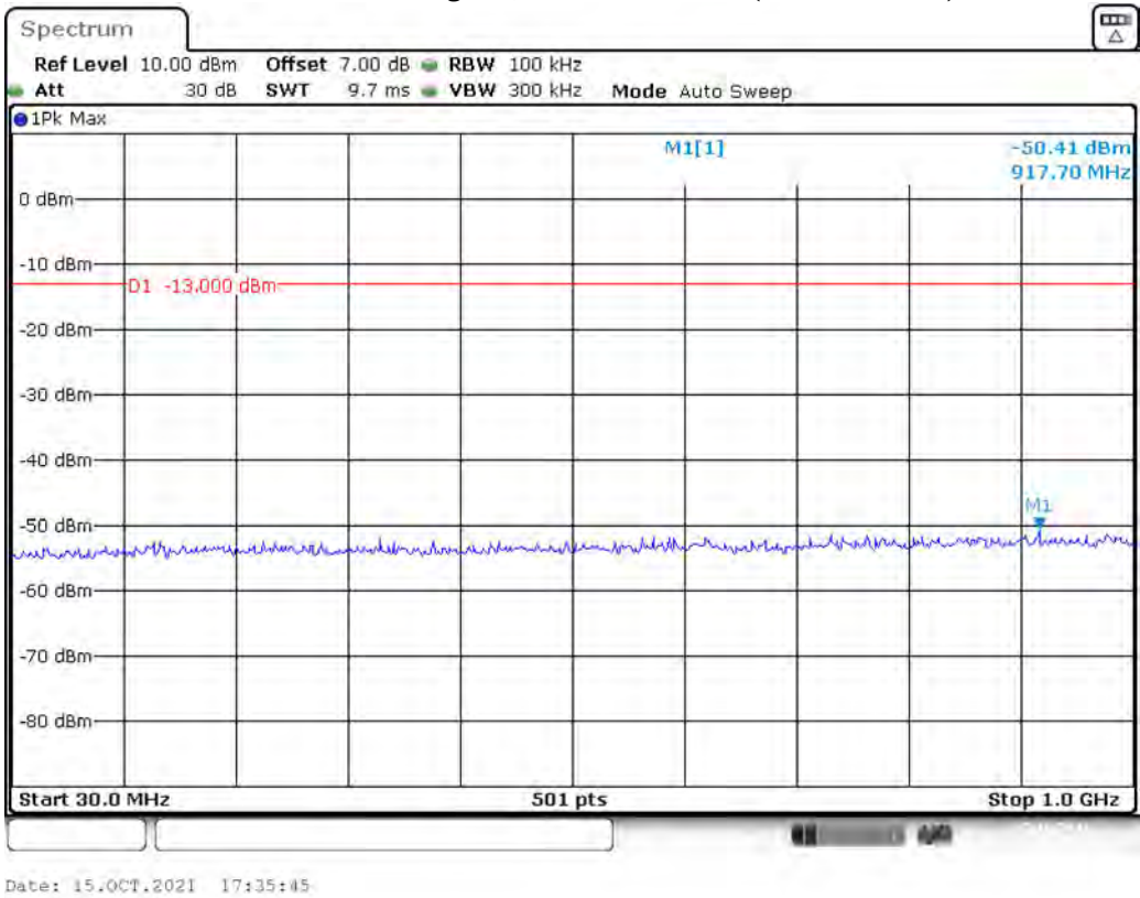
Band 4_20 MHz_High_QPSK_RB100#0_1(30MHz-1GHz)
