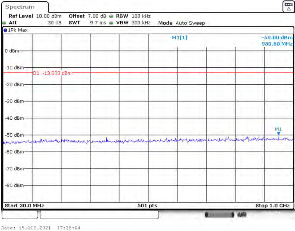
Band 4_10 MHz_Low_QPSK_RB50#0_1(30MHz-1GHz)
