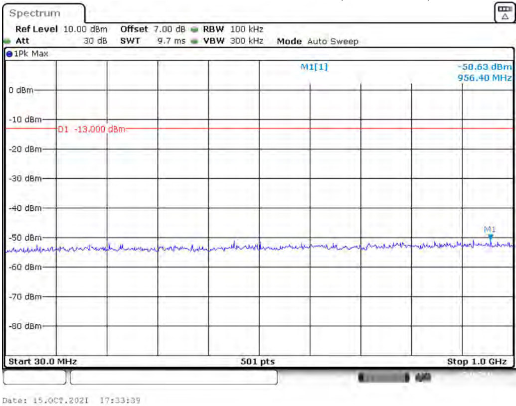
Band 4_20 MHz_Low_QPSK_RB100#0_1(30MHz-1GHz)
