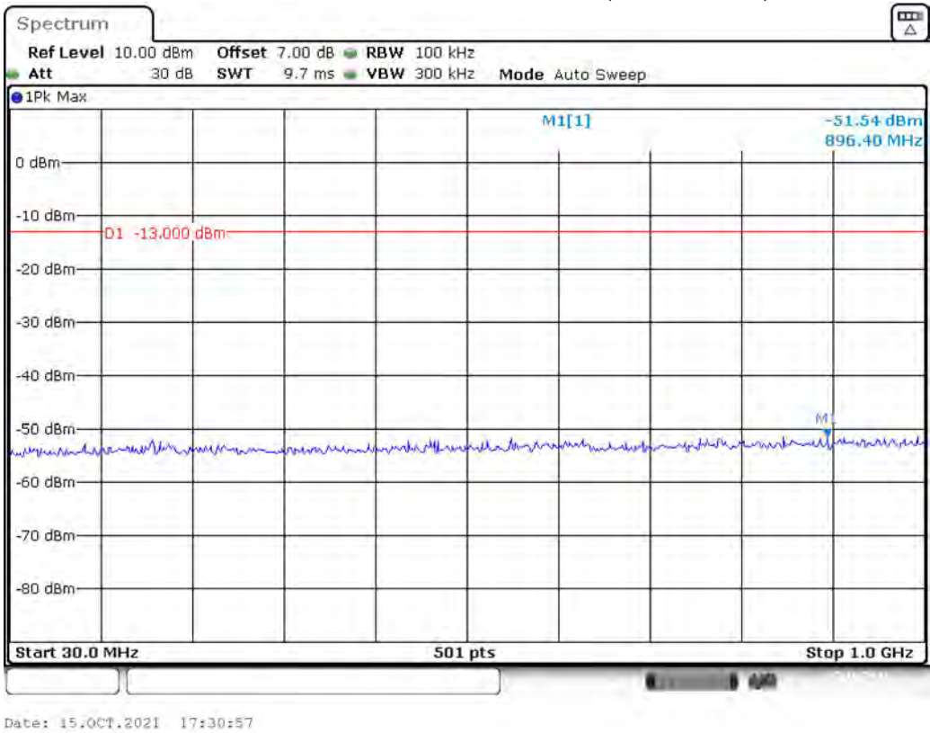
Band 4_15 MHz_Low_QPSK_RB75#0_1(30MHz-1GHz)
