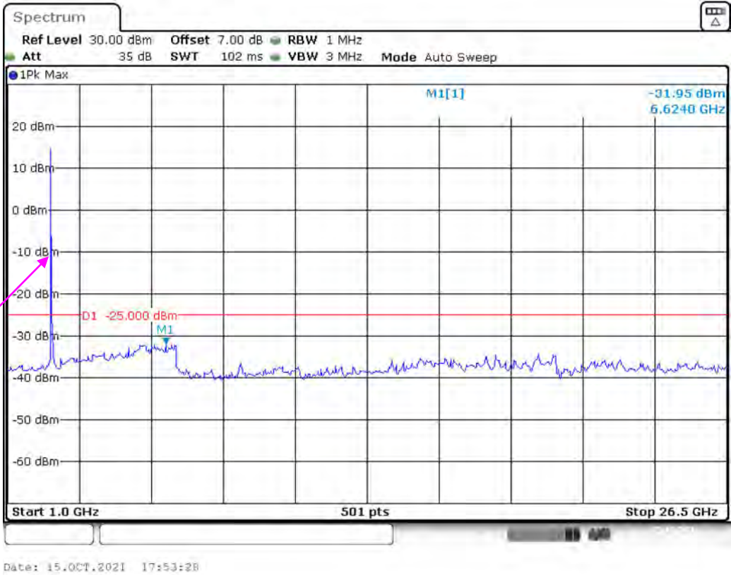
Band 7_10 MHz_High_QPSK_RB50#0_2(1GHz-26.5GHz)
