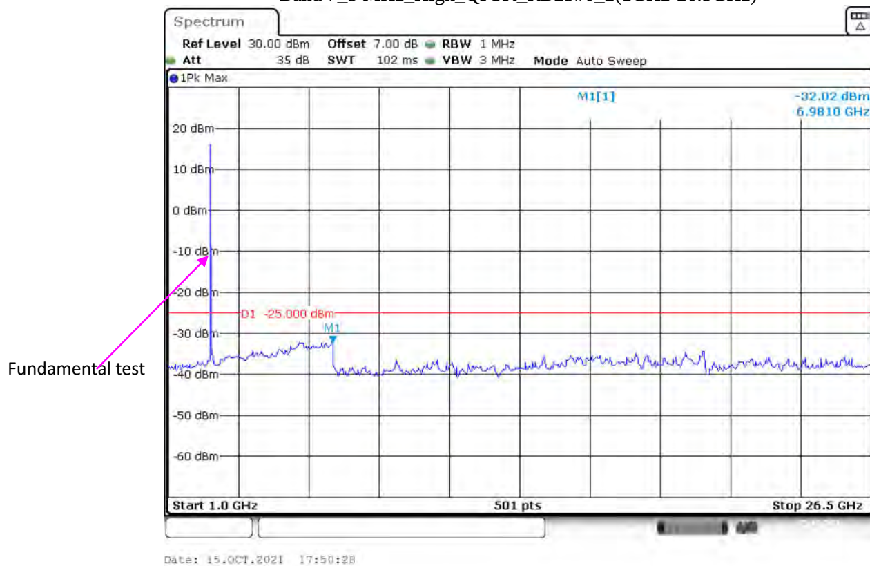
Band 7_5 MHz_High_QPSK_RB25#0_2(1GHz-26.5GHz)
