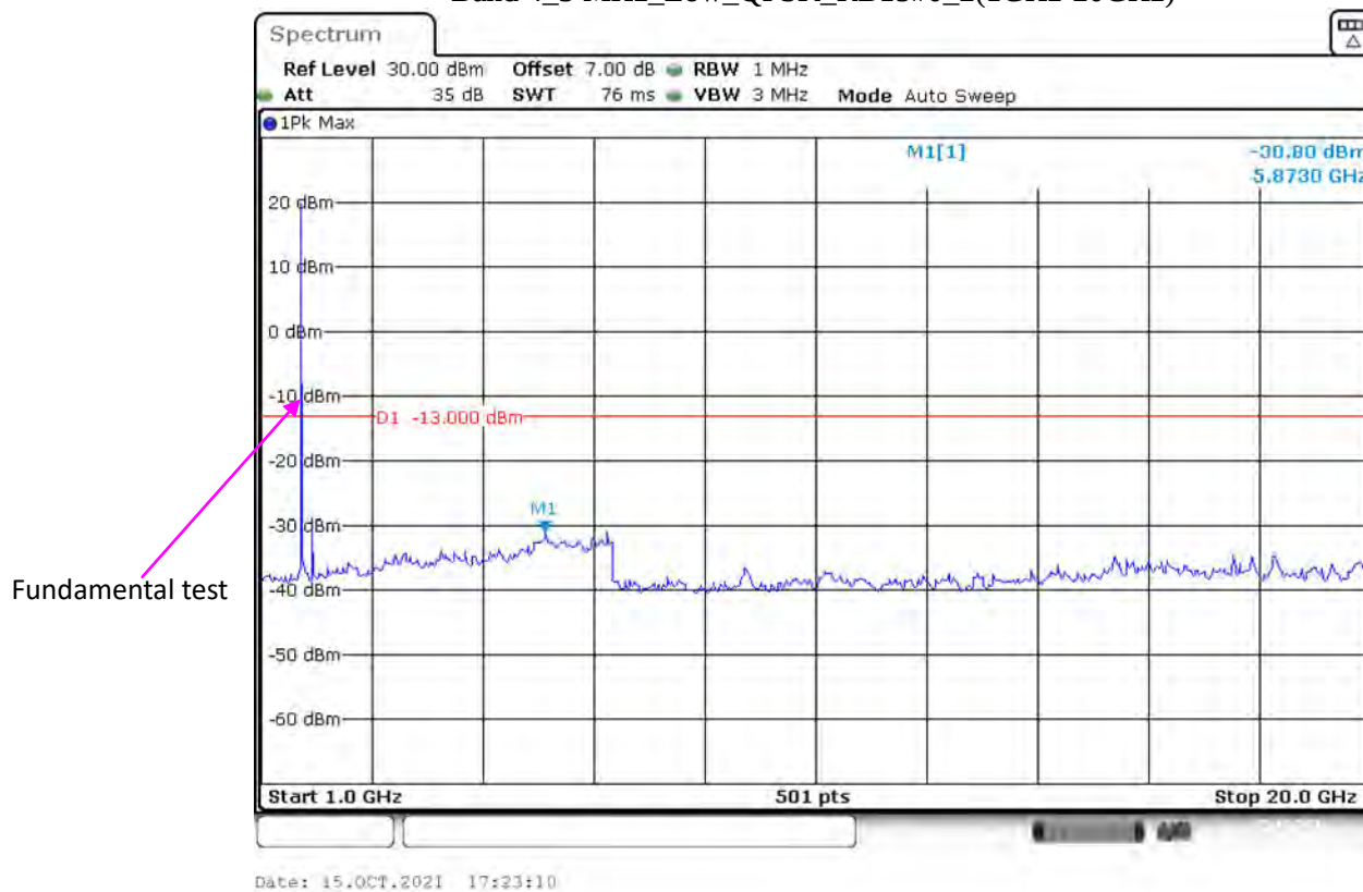
Band 4_3 MHz_Low_QPSK_RB15#0_2(1GHz-20GHz)
