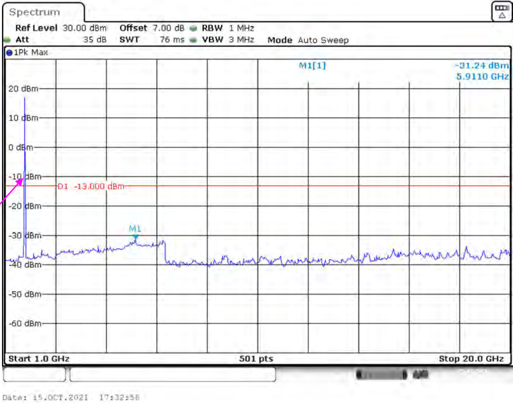
Band 4_15 MHz_High_QPSK_RB75#0_2(1GHz-20GHz)
