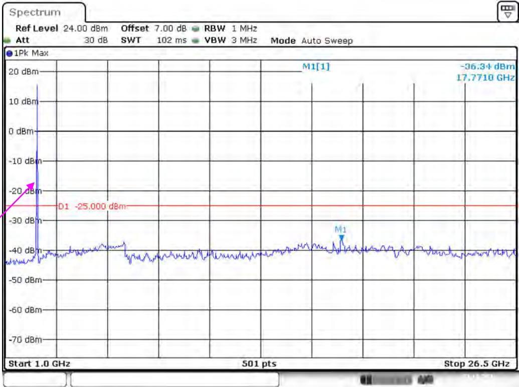
Band 38_15 MHz_Middle_QPSK_RB75#0_2(1GHz-26.5GHz)
