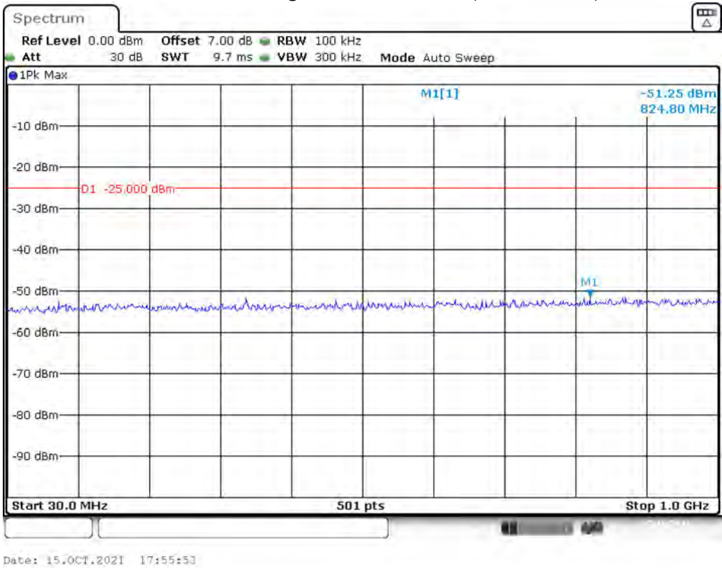
Band 7_15 MHz_High_QPSK_RB75#0_1(30MHz-1GHz)
