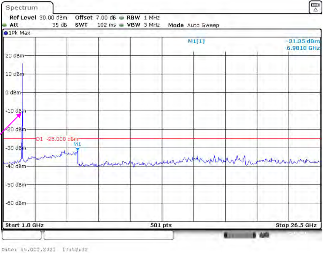
Band 7_10 MHz_Middle_QPSK_RB50#0_2(1GHz-26.5GHz)
