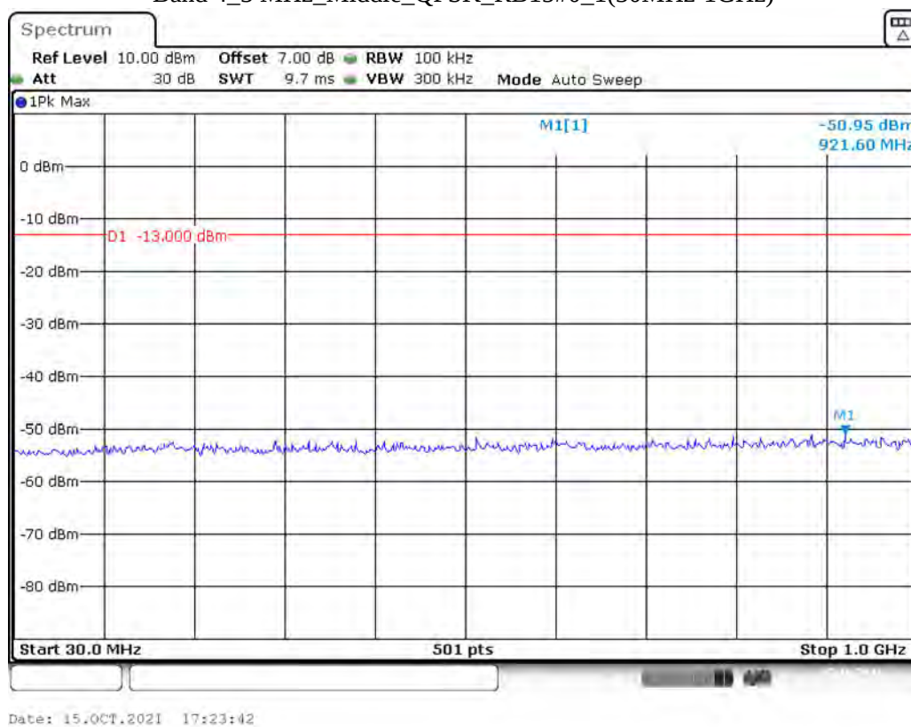
Band 4_3 MHz_Middle_QPSK_RB15#0_1(30MHz-1GHz)
