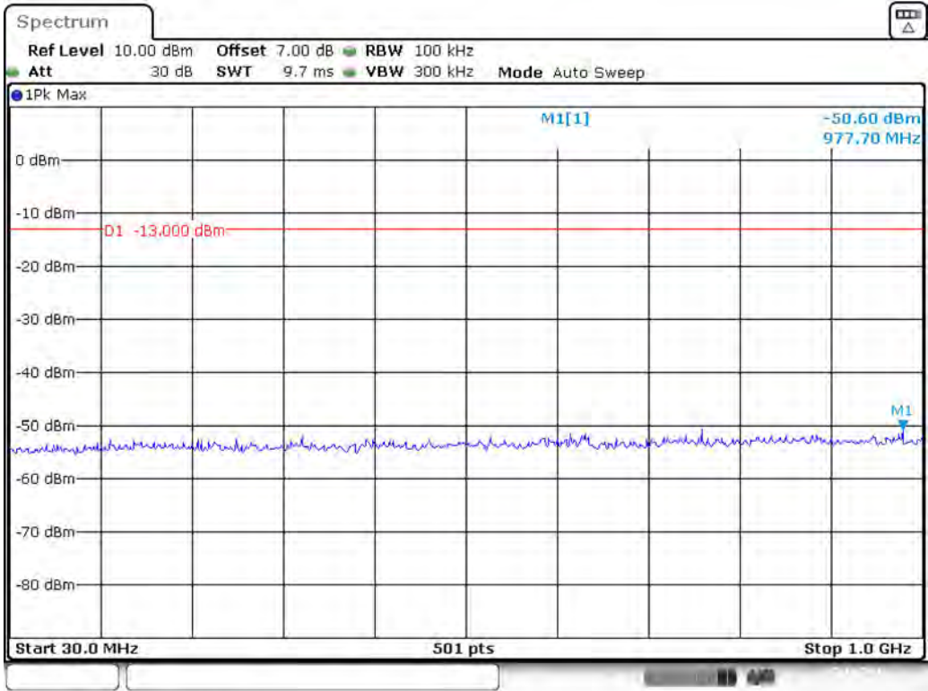
Band 4_15 MHz_Middle_QPSK_RB75#0_1(30MHz-1GHz)
