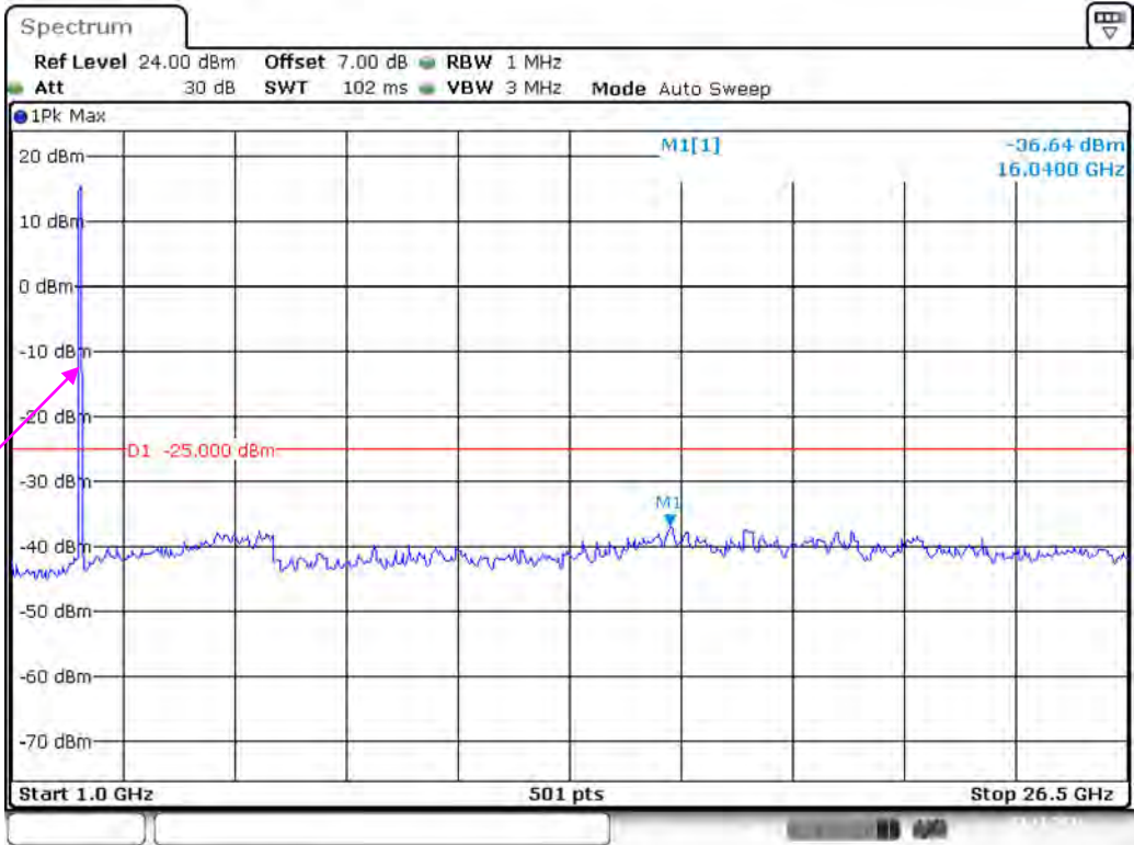
Band 38_10 MHz_Low_QPSK_RB50#0_2(1GHz-26.5GHz)
