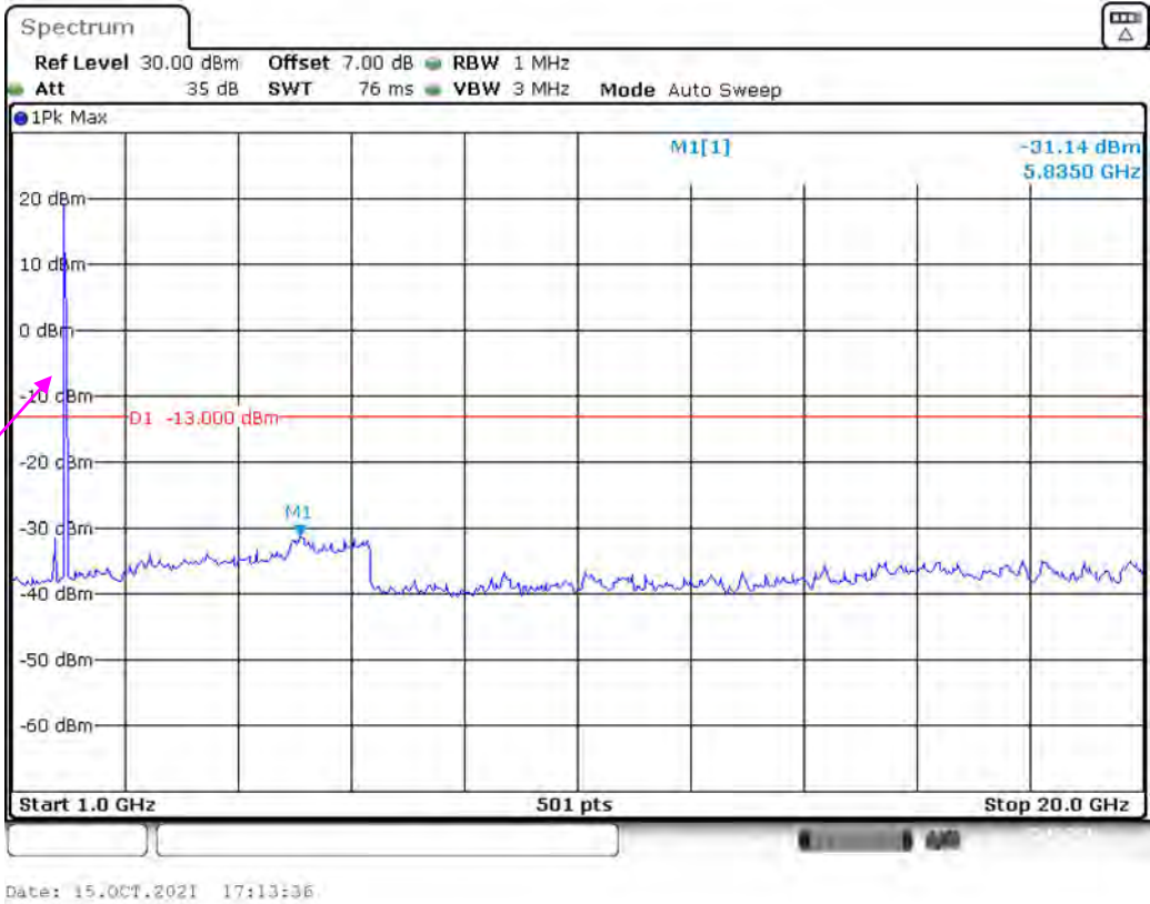
Band 2_10 MHz_High_QPSK_RB50#0_2(1GHz-20GHz)
