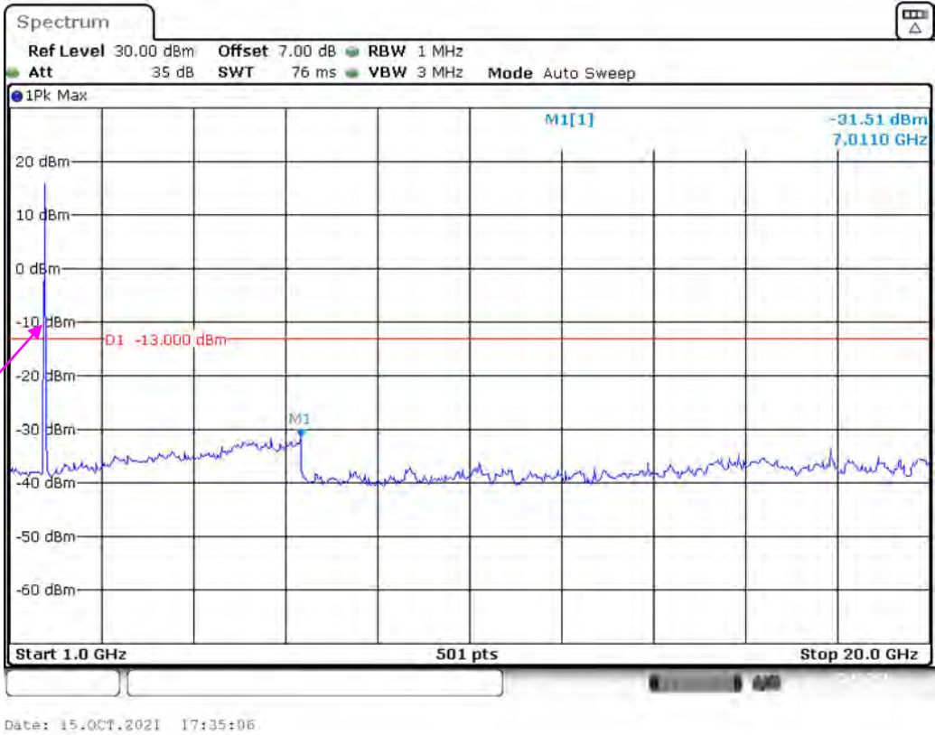
Band 4_20 MHz_Middle_QPSK_RB100#0_2(1GHz-20GHz)
