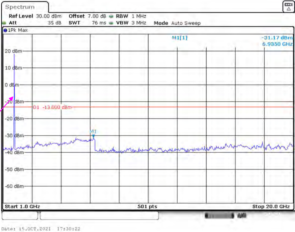
Band 4_10 MHz_High_QPSK_RB50#0_2(1GHz-20GHz)
