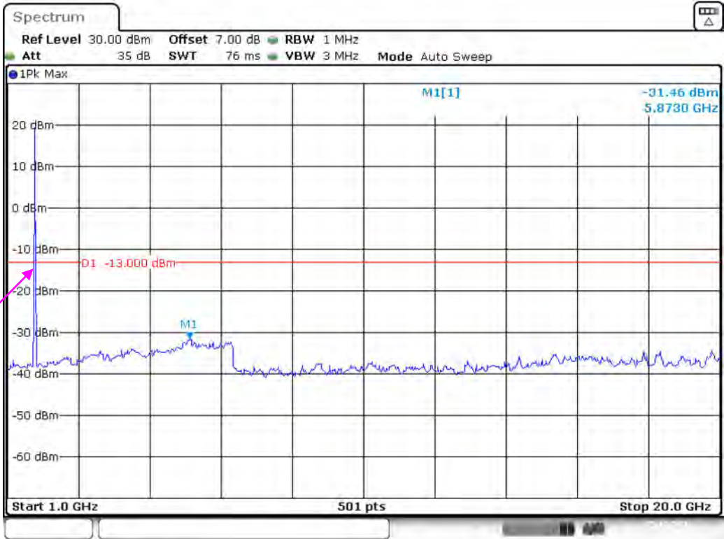
Band 66_10 MHz_Middle_QPSK_RB50#0_2(1GHz-20GHz)
