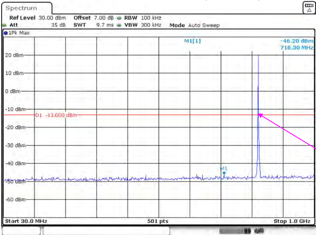
Band 5_1.4 MHz_Low_QPSK_RB6#0_1(30MHz-1GHz)
