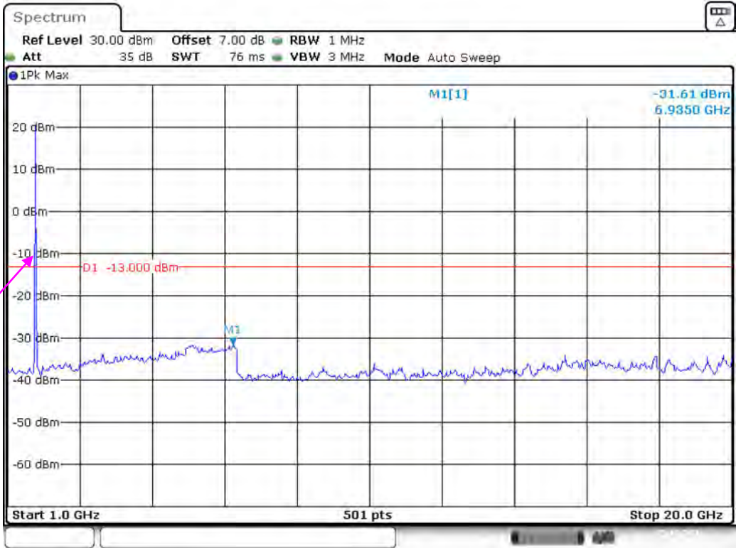
Band 4_3 MHz_High_QPSK_RB15#0_2(1GHz-20GHz)
