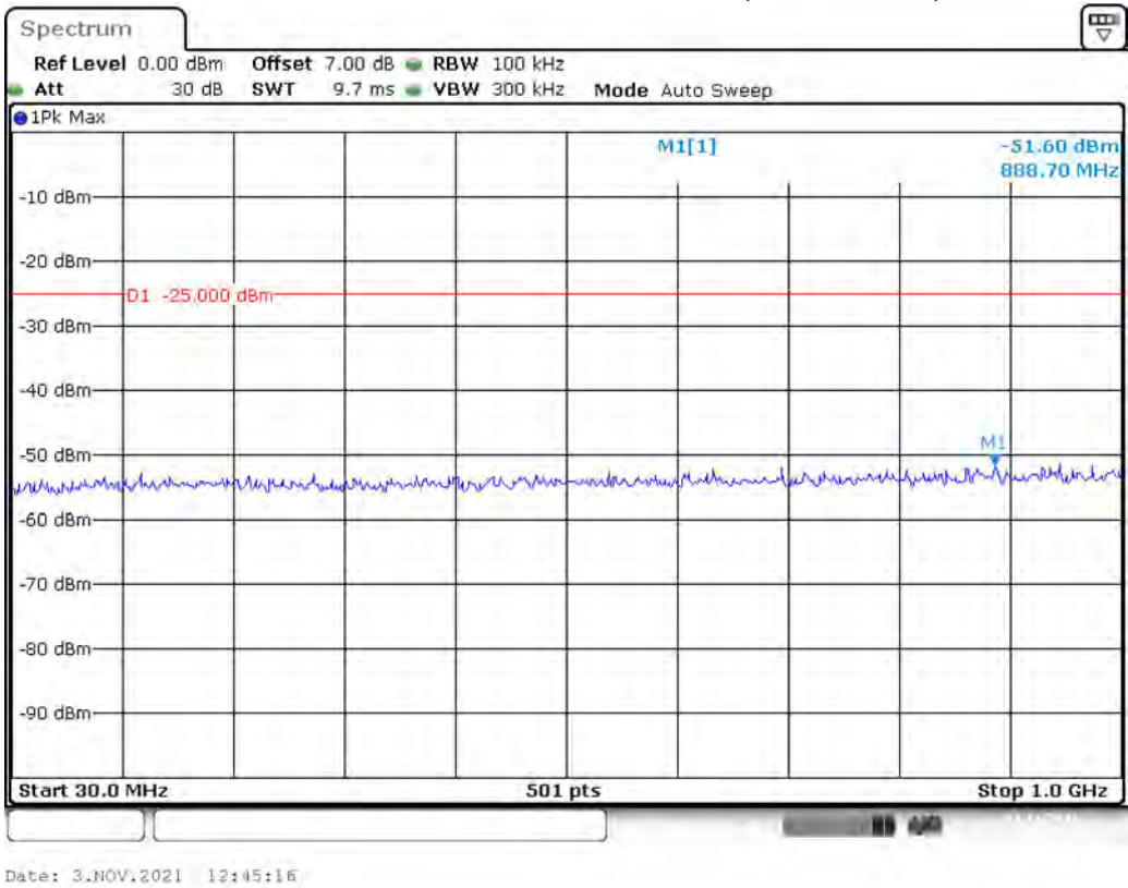
Band 38_15 MHz_Low_QPSK_RB75#0_1(30MHz-1GHz)
