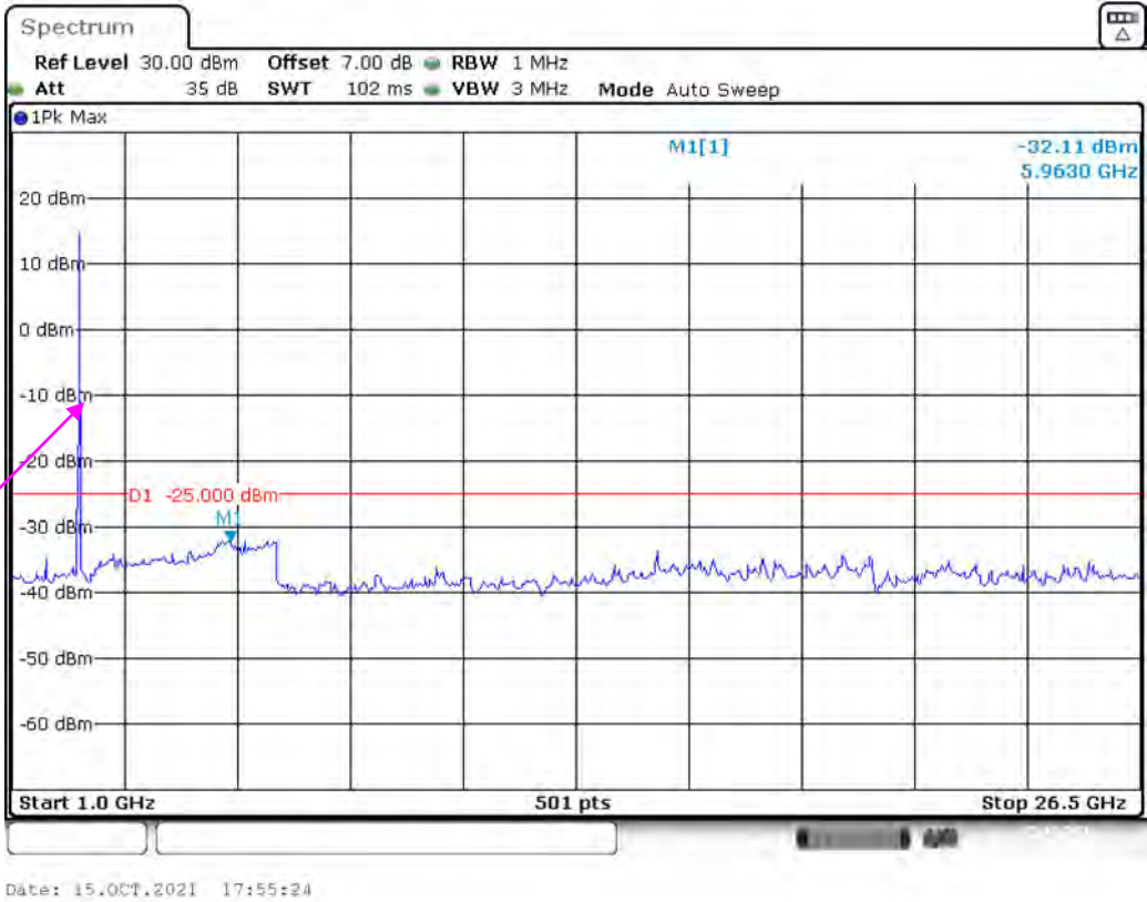
Band 7_15 MHz_Middle_QPSK_RB75#0_2(1GHz-26.5GHz)
