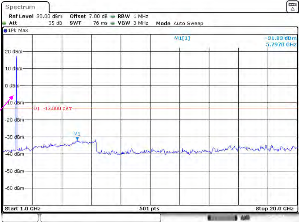
Band 2_20 MHz_Middle_QPSK_RB100#0_2(1GHz-20GHz)
