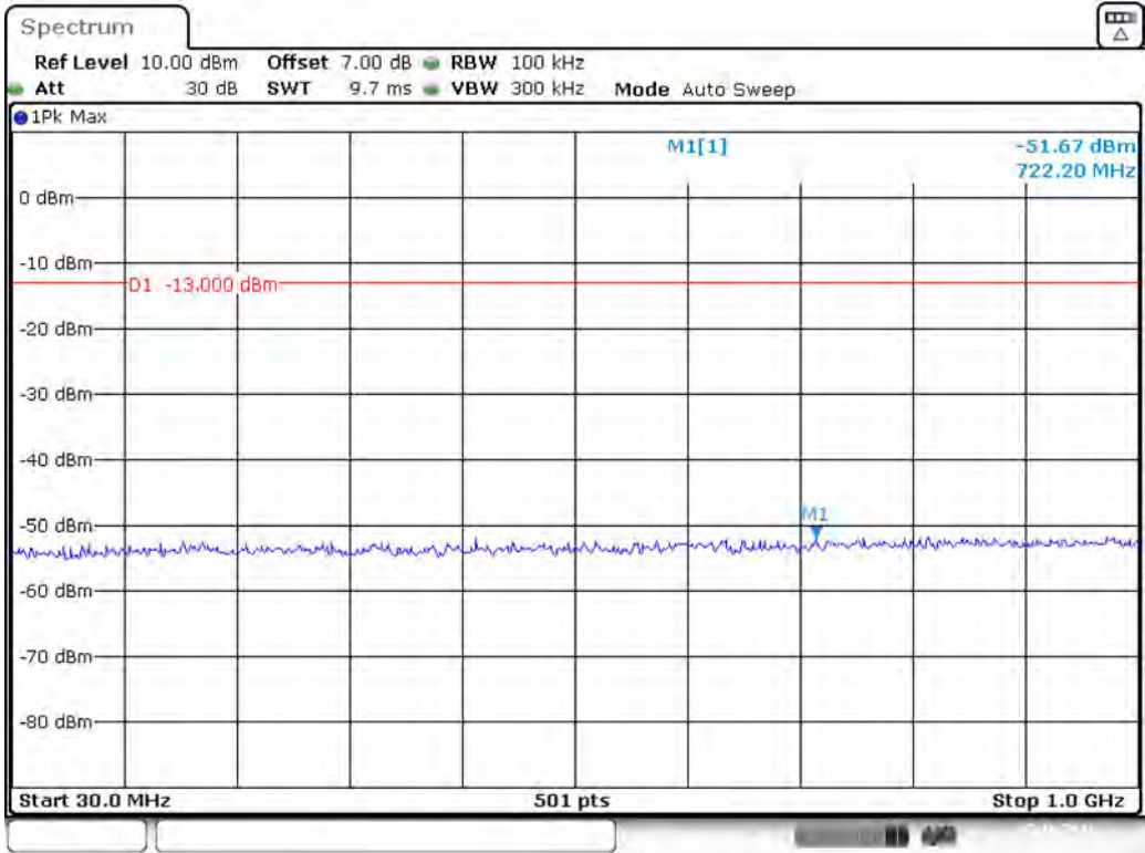
Band 4_20 MHz_Middle_QPSK_RB100#0_1(30MHz-1GHz)
