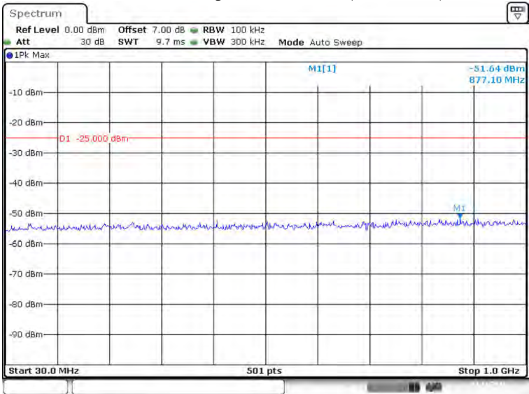
Band 38_15 MHz_High_QPSK_RB75#0_1(30MHz-1GHz)
