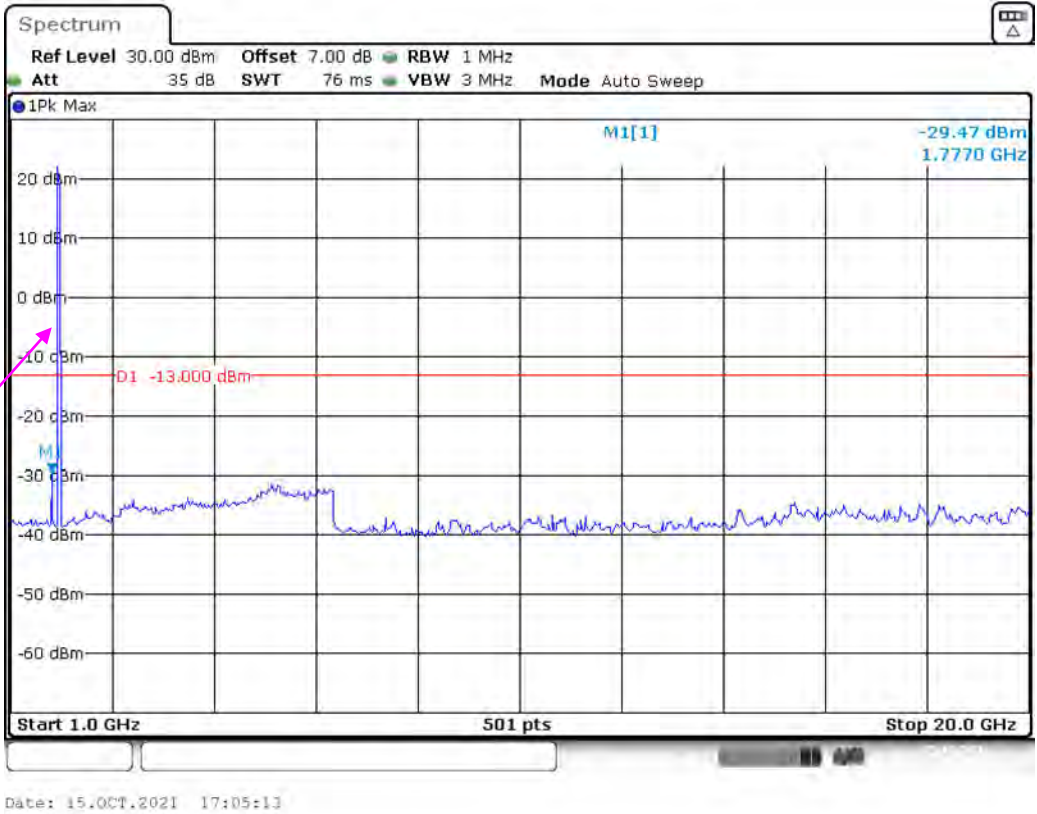
Band 2_1.4 MHz_High_QPSK_RB6#0_2(1GHz-20GHz)
