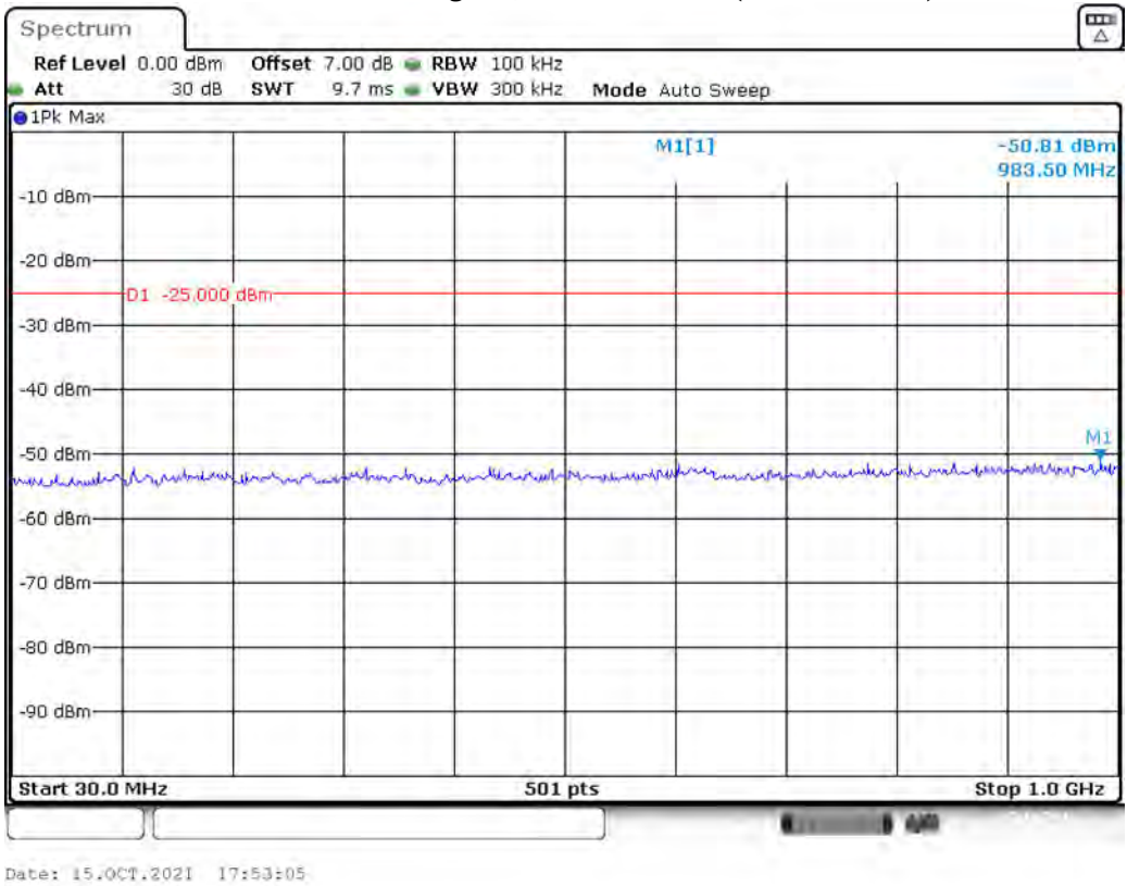
Band 7_10 MHz_High_QPSK_RB50#0_1(30MHz-1GHz)
