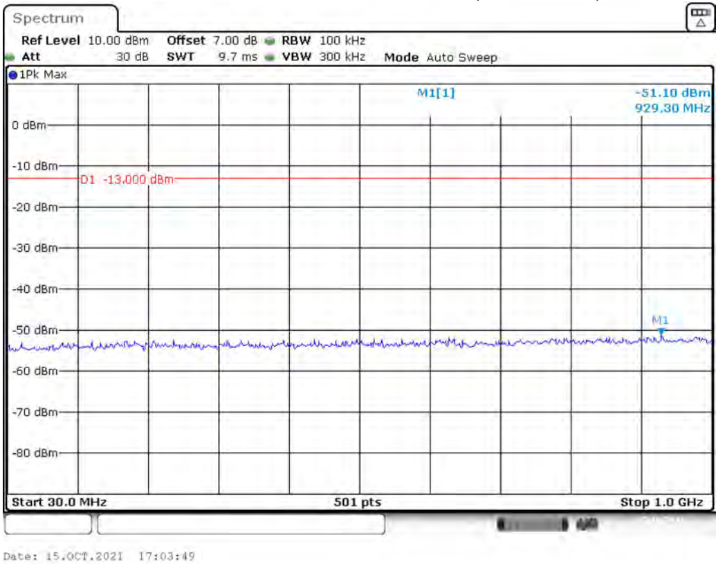
Band 2_1.4 MHz_Middle_QPSK_RB6#0_1(30MHz-1GHz)
