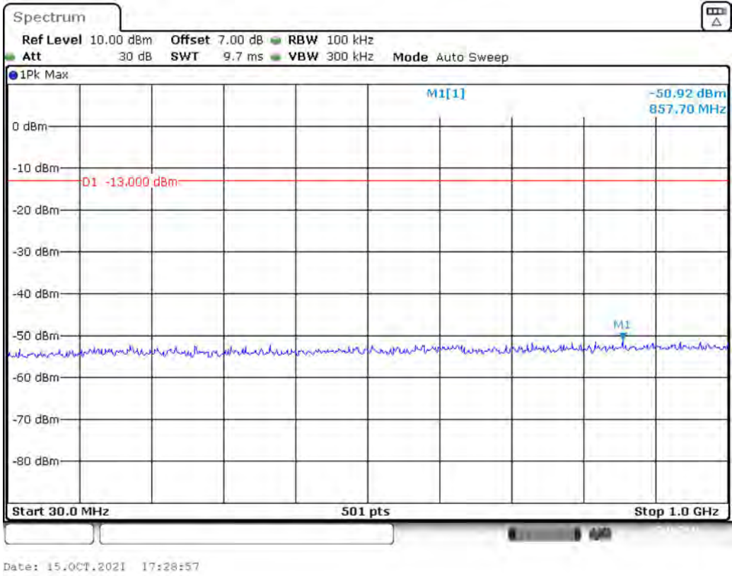
Band 4_10 MHz_Middle_QPSK_RB50#0_1(30MHz-1GHz)
