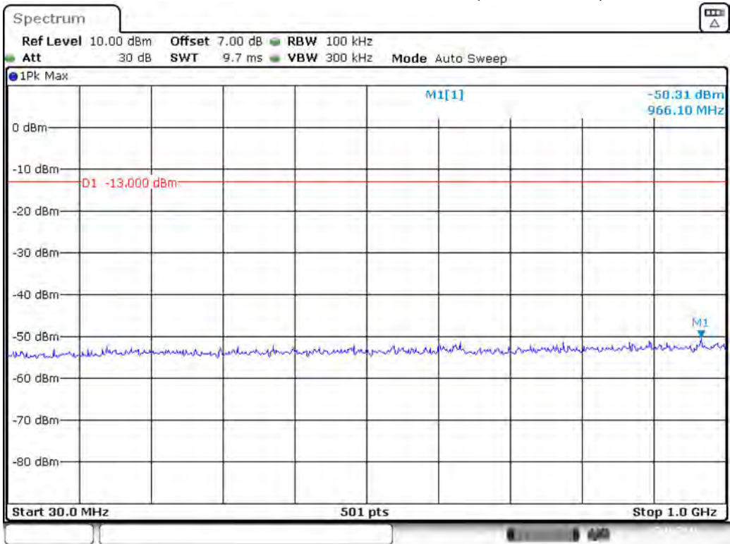
Band 66_3 MHz_Low_QPSK_RB15#0_1(30MHz-1GHz)
