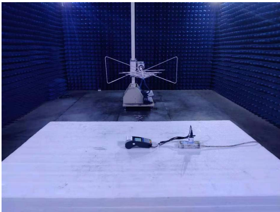
Photo of Radiated Emission Measurement (30MHz-1GHz) For adapter1
