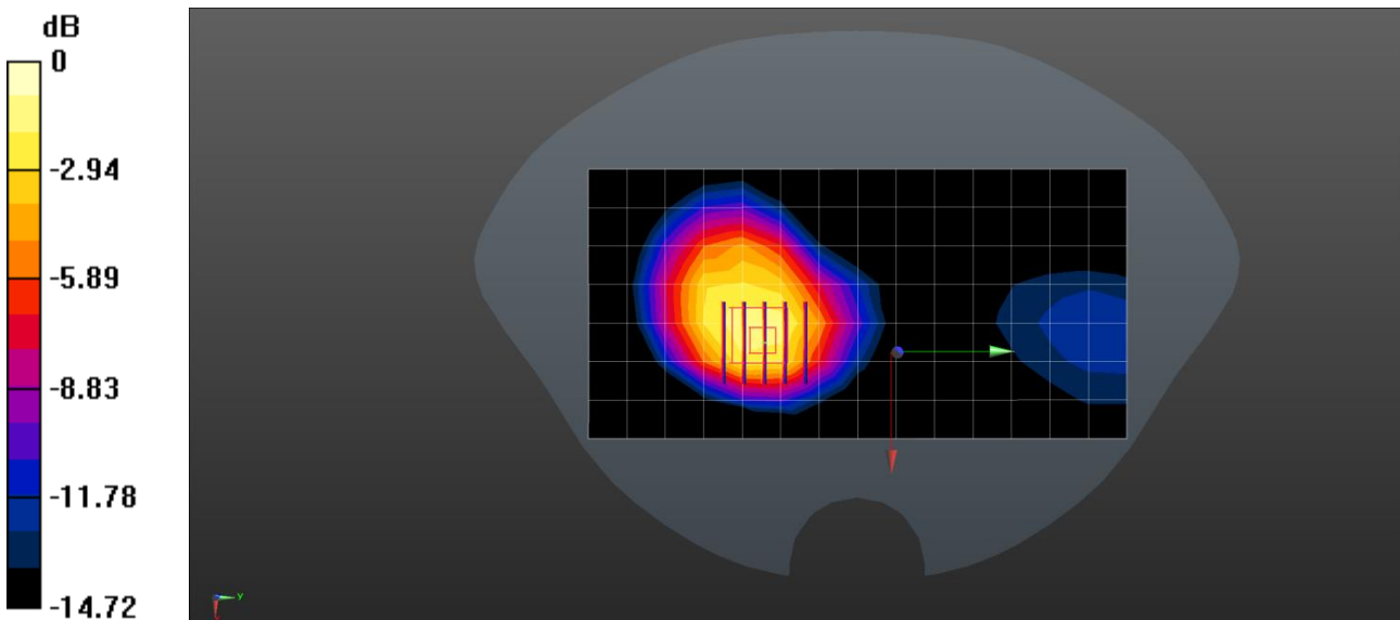
0 dB = 1.47 W/kg = 1.67 dBW/kg
