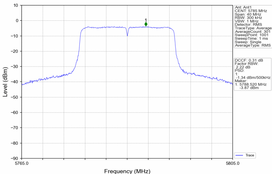
802.11ac(VHT20)_MCH_5785MHz_Ant1_NTNV
