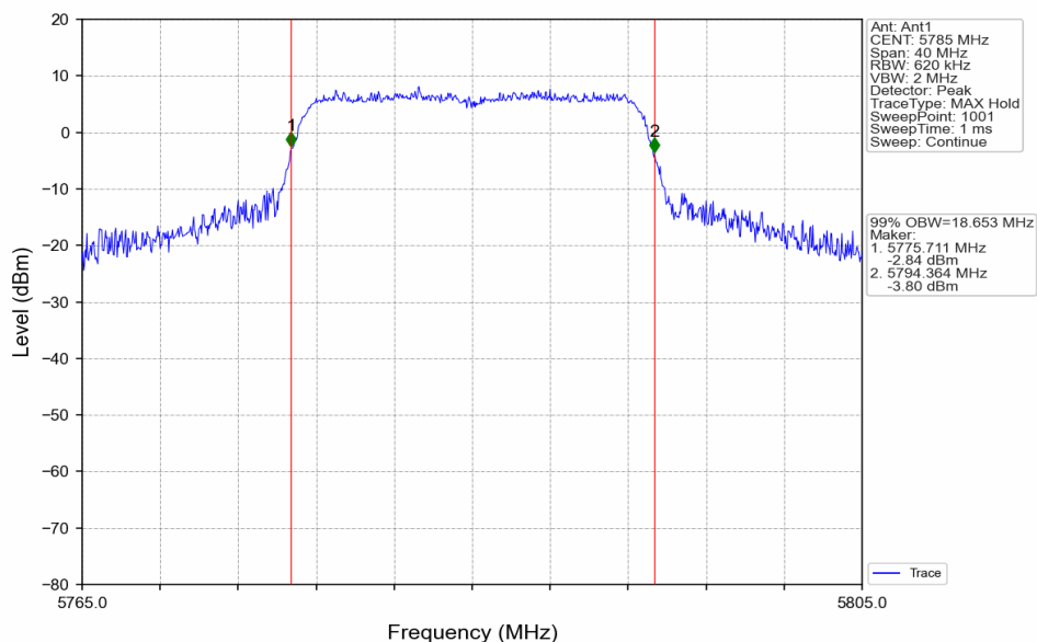
802.11ac(VHT20)_MCH_5785MHz_Ant1_NTNV
