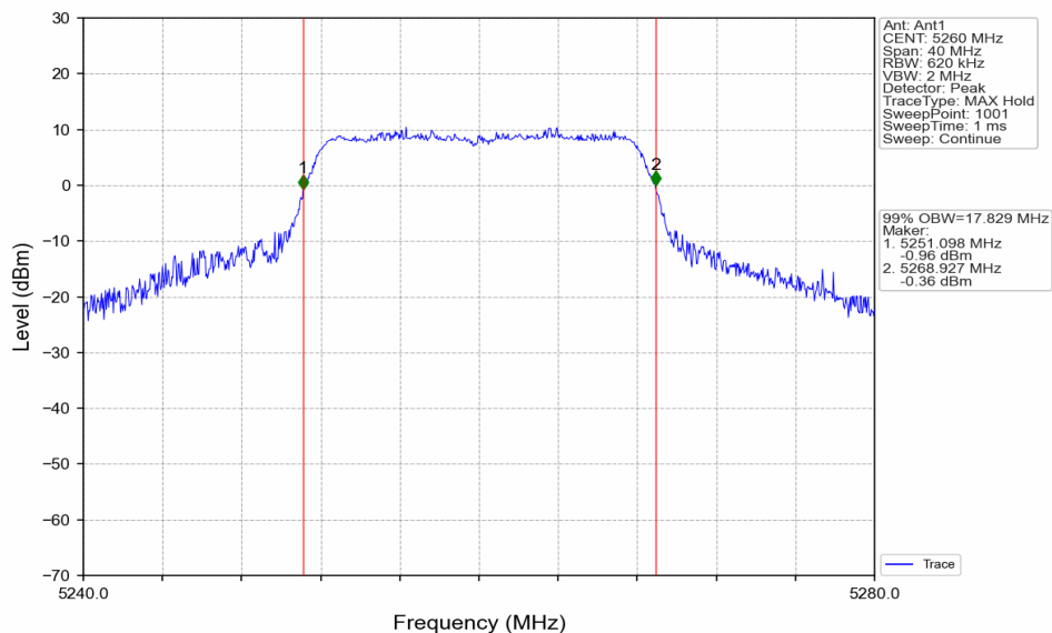
802.11a_LCH_5260MHz_Ant1_NTNV
