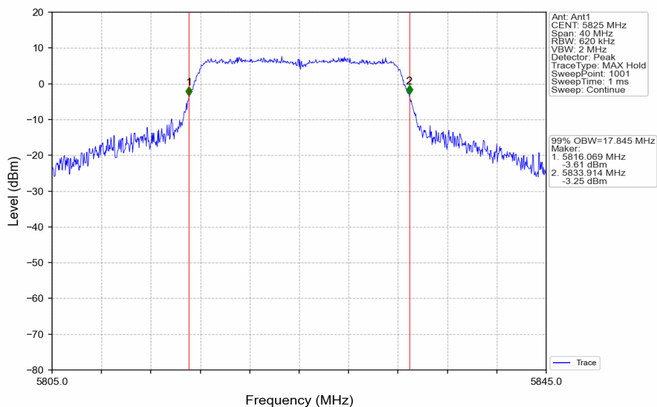
802.11a_HCH_5825MHz_Ant1_NTNV
