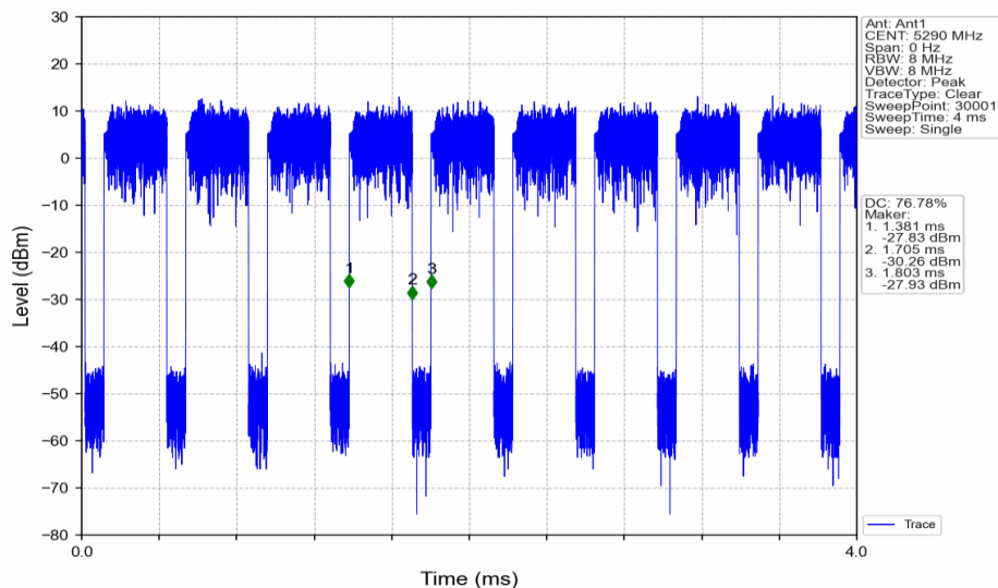
802.11ac(VHT80)_MCH_5290MHz_Ant1_NTNV
