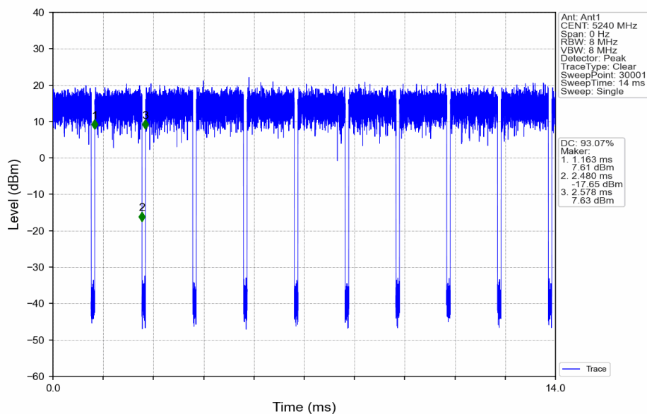
802.11ac(VHT20)_HCH_5240MHz_Ant1_NTNV
